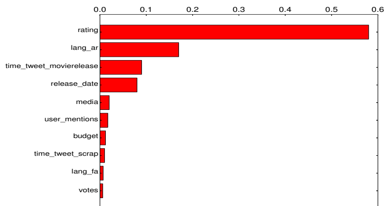
(C) Relevance of features after cleaning the retweet effect and removing user features.
