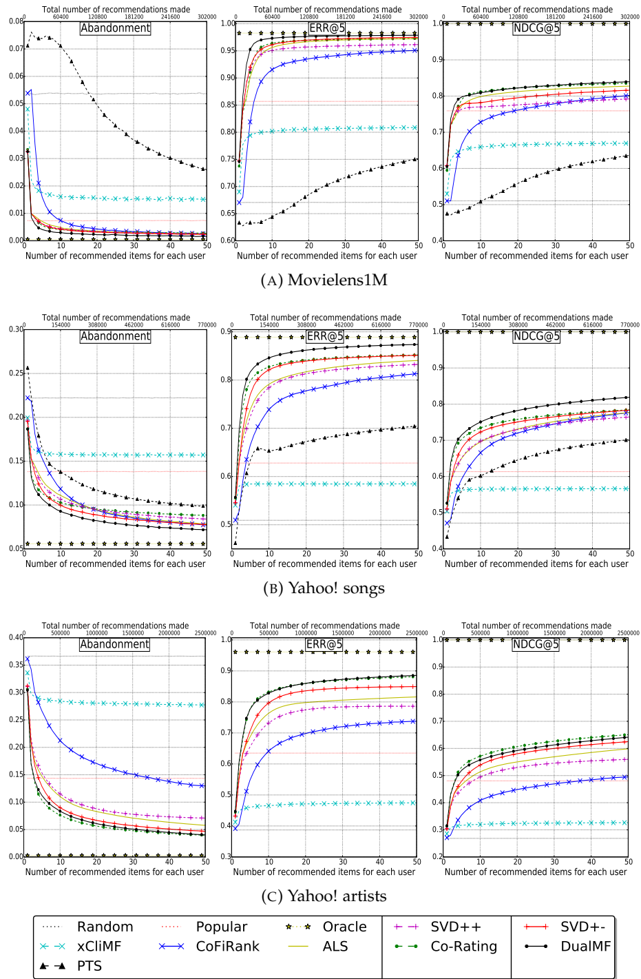
FIGURE 4.2: Evaluation of algorithms on three datasets and three metrics with the ERR click model (from the left column to the right one: Abandonment, ERR@5, NDCG@5).
