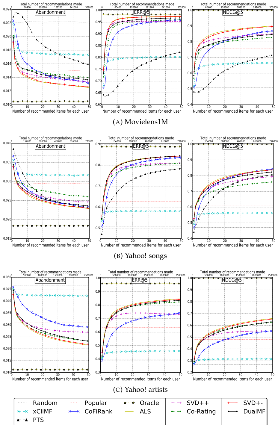
FIGURE 4.5: Evaluation of algorithms on three datasets and three metrics with the almost random click model (from the left column to the right one: Abandonment, ERR@5, NDCG@5).
