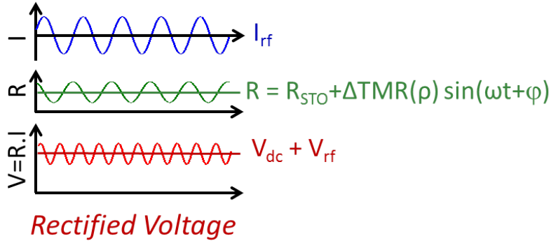
FIGURE 7.1: Principle of the spin-diode rectification voltage
