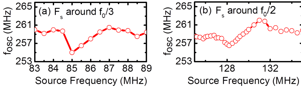
FIGURE 4.9: Oscillator frequency f_{osc} vs external source frequency F_s around f_0/3 (a), f_0/2 (b) for I_{rf} = 2 mA (at H=0 and I_{dc} = +11 mA and \varnothing = 300 nm)
