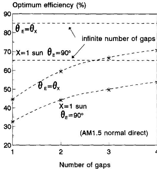
Figure 1.7 – Conversion efficiency limits as a function of the number of junction under AM1.5 irradiation extracted from [7]
