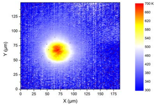
(c) Temperature of emission of the sample 2757 under 22000 suns illumination
