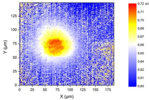
(e) \Delta\mu of the sample 2757 under 22000 suns illumination
