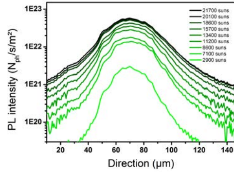
(b) Spectrally integrated PL along X direction at Y =Barycenter of the left corresponding map at different illumination powers
