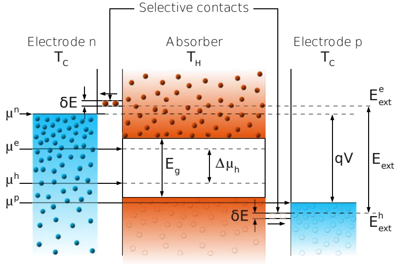
Figure 1.8 – Schematic of a HCSC extracted from [8]
