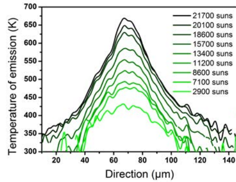
(d) Temperature of emission along X direction at Y =Barycenter of the top/left PL map at different illumination powers
