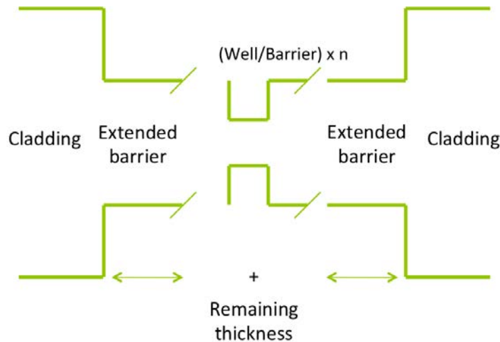
Figure 2.7 – Simplified band diagram structure of samples studied
