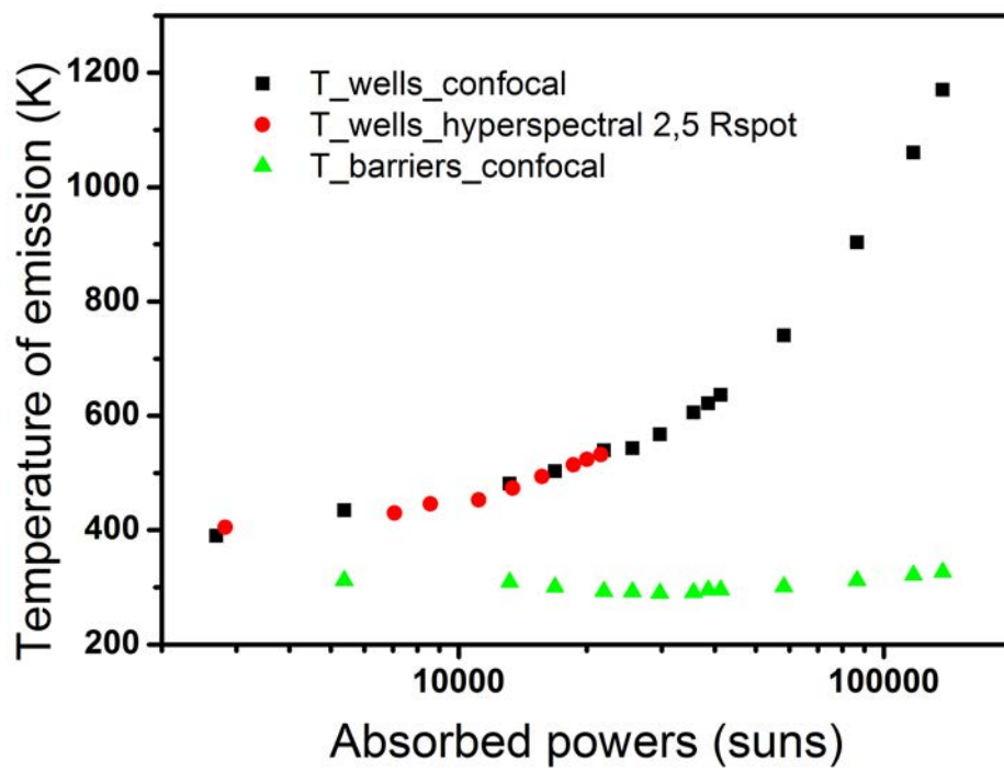
Figure B.1 – Local temperature of emission
