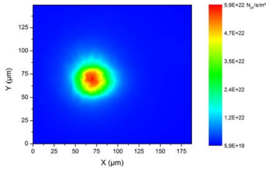
(a) Spectrally integrated PL map of the sample 2757 under 22000 suns illumination
