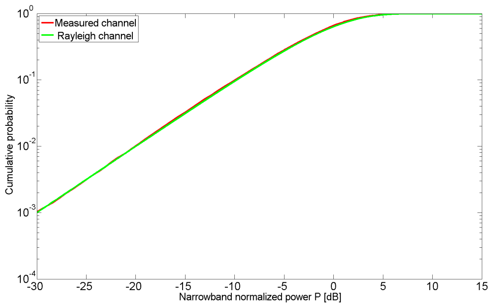
Figure 4.8 – Comparison of measured and Rayleigh fading CDFs [dB].
