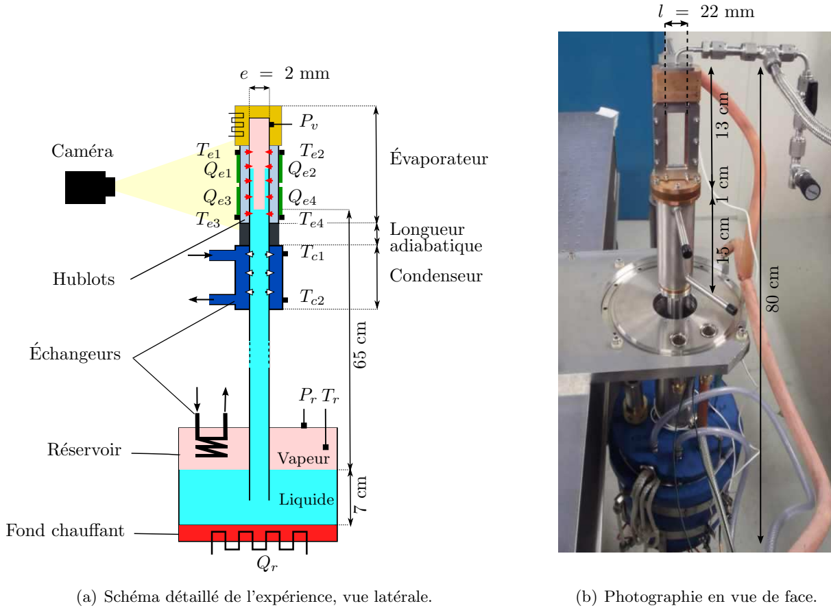
FIGURE 2.1. – Installation expérimentale.
