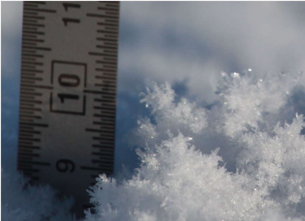
Figure B.2: Picture of the small ice crystals at Dome C during the time lapse of the frost deposition during 24 hours
