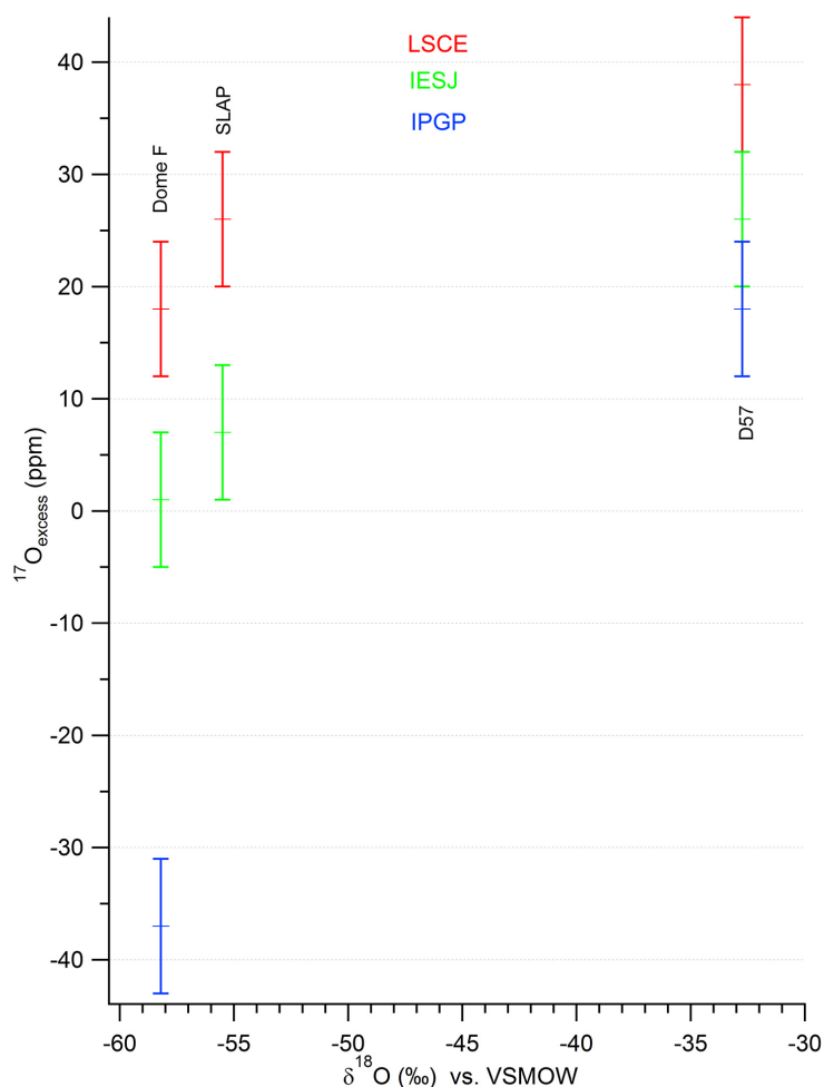
Figure 3.2: ^{17}\text{O} – excess values vs \delta^{18}\text{O} for water standards measured at LSCE, IESJ and IPGP for intercalibration (Winkler, 2012)
