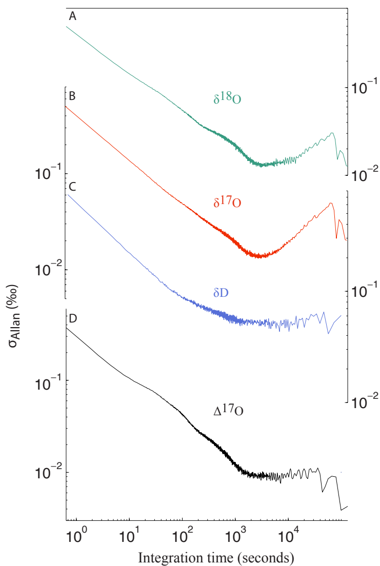
Figure 3.14: Allan standard deviation for water isotopic composition measured of a Picarro L2140-i: (A) \delta^{18}O : green, (B) \delta^{17}O : red, (C) \delta D : blue and (D) ^{17}O - excess : black. Modified from Steig et al. [2014] .
