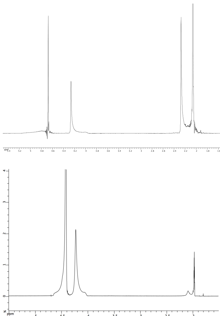
Figure 8.1: 1D 1 H spectra of the acetonitrile-water mixture; left: protonated acetonitrile-water 70% - 30% vv at 0 °C; right: deuterated acetonitrile-water 70% - 30% vv at 6 °C.
