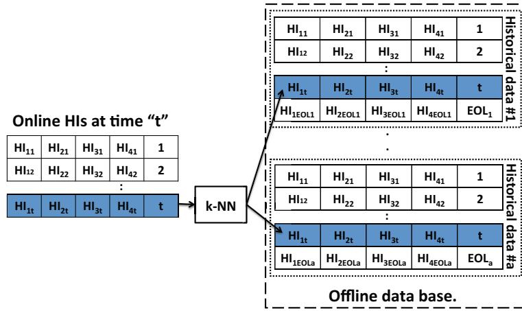
Figure 5.7: Finding the most similar offline HIs to the test HIs. The algorithm assigns the EOL of the selected HIs to the test HIs to calculate the RUL.
