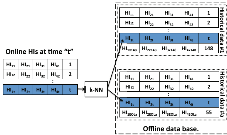
Figure 5.8: Classification can lead to a huge RUL estimation error.
