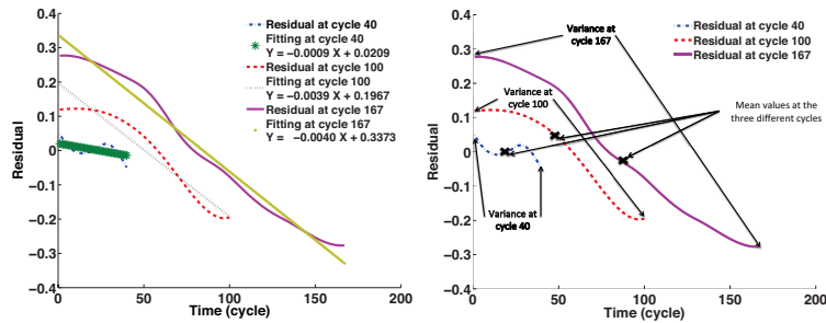
(a) HI using slope and intersect. (b) HI using mean and variance.
