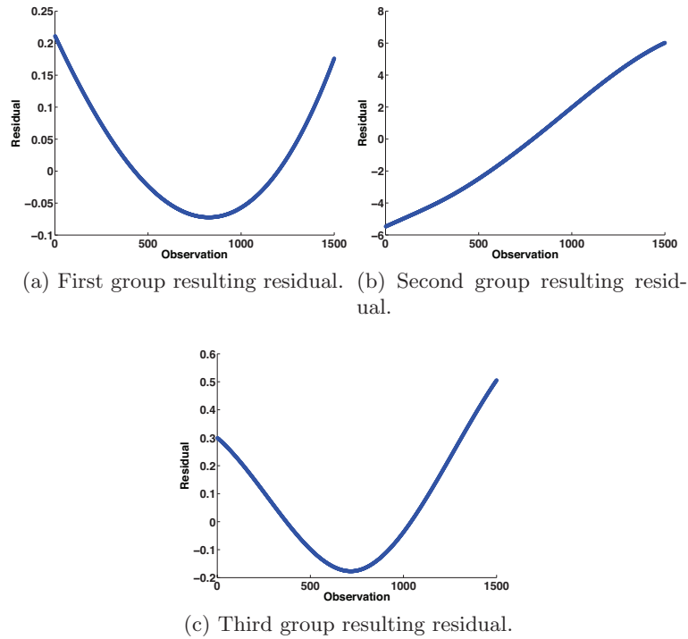
Figure 4.22: Residual extracted from the three groups first components.
