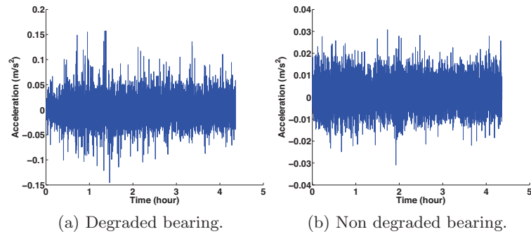
Figure 4.23: Vibration signals acquired from two bearings.
