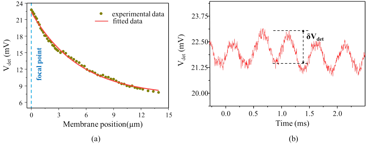
Figure 3.21: (a) Mapping the z-axis: position of the membrane along z-axis vs. detected voltage at the BHD output with no membrane excitation, (b) oscillation of the output voltage while the membrane (placed at the focal point) is resonantly excited, the fluctuation is directly related to the membrane displacement.
