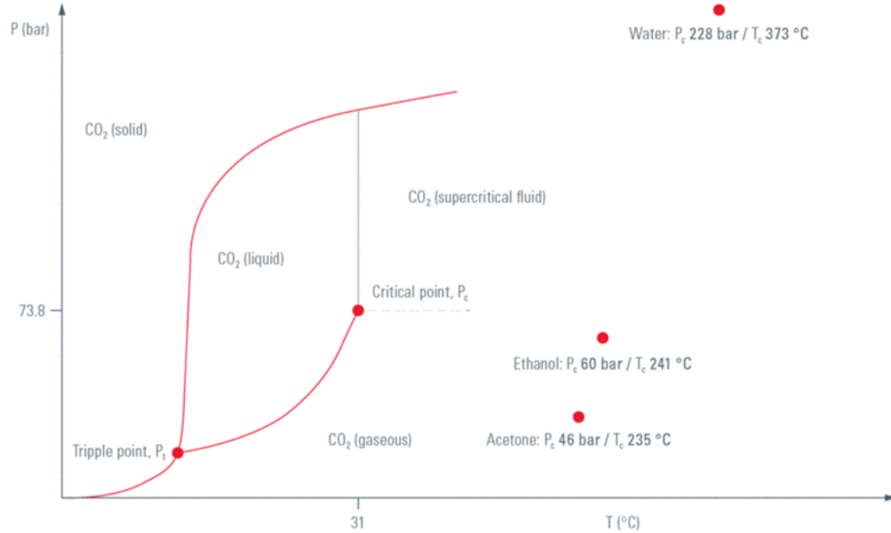
Figure 3.13: Phase diagram showing the supercritical transition of CO_2 [89].
