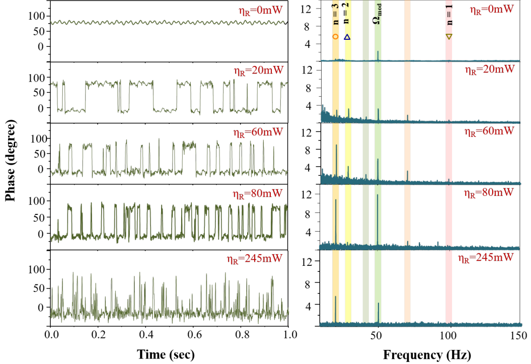
Figure 5.21: (a) Time evolution of phase switching with increase in the amplitude noise (at 50Hz of modulation frequency); we observe the best situation of synchronization for a amplitude noise of 80mW , (b) evolution of the corresponding FFT spectra; we observe several harmonics along with the main resonance peak at 50Hz .
