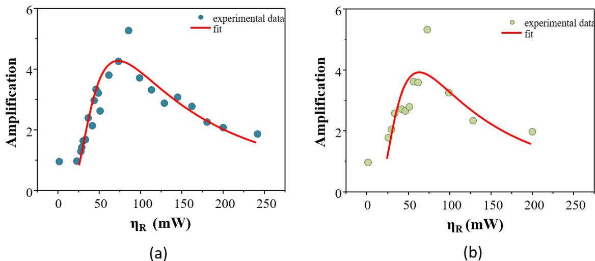
Figure 5.22: Amplification by stochastic resonance with amplitude modulation and noise for a modulation frequency of 50Hz and for a modulation depth m of (a) 10% and (b) 20%.
