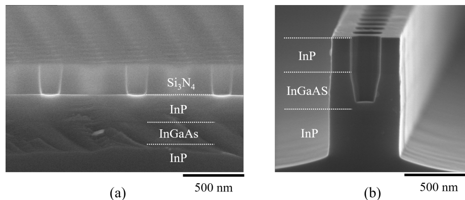
Figure 3.10: SEM picture of a photonic crystal lattice cross-section after its transfer into (a) Si_3N_4 mask and (b) into a InP layer.
