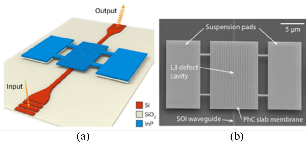
Figure 6.1: (a) Schematic of the PhC membrane and waveguide system; light is injected through one end of the waveguide and it interacts with the PhC cavity and the modified field is collected at the other end of the waveguide, (b) An scanning electron micrograph of the fabricated membrane-waveguide structure where the membrane is suspended about 230nm above the Si waveguide.
