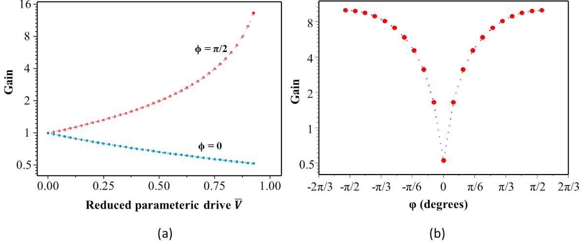
Figure 4.18: (a) Variation of parametric gain with the parametric drive under two separate phase differences \phi = 0 and \phi = \pi/2 (b) Variation of parametric gain with the phase difference between the resonant drive and parametric pump under a constant reduced parametric drive \bar{V} = 0.9 .
