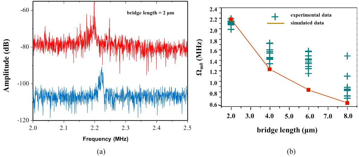
Figure 2.10: (a) Mechanical noise spectra of two different membranes with identical geometry separated by an offset, (b) plot of experimentally and simulated (FEM simulation) eigen-frequency ( \Omega_{m0} ).
