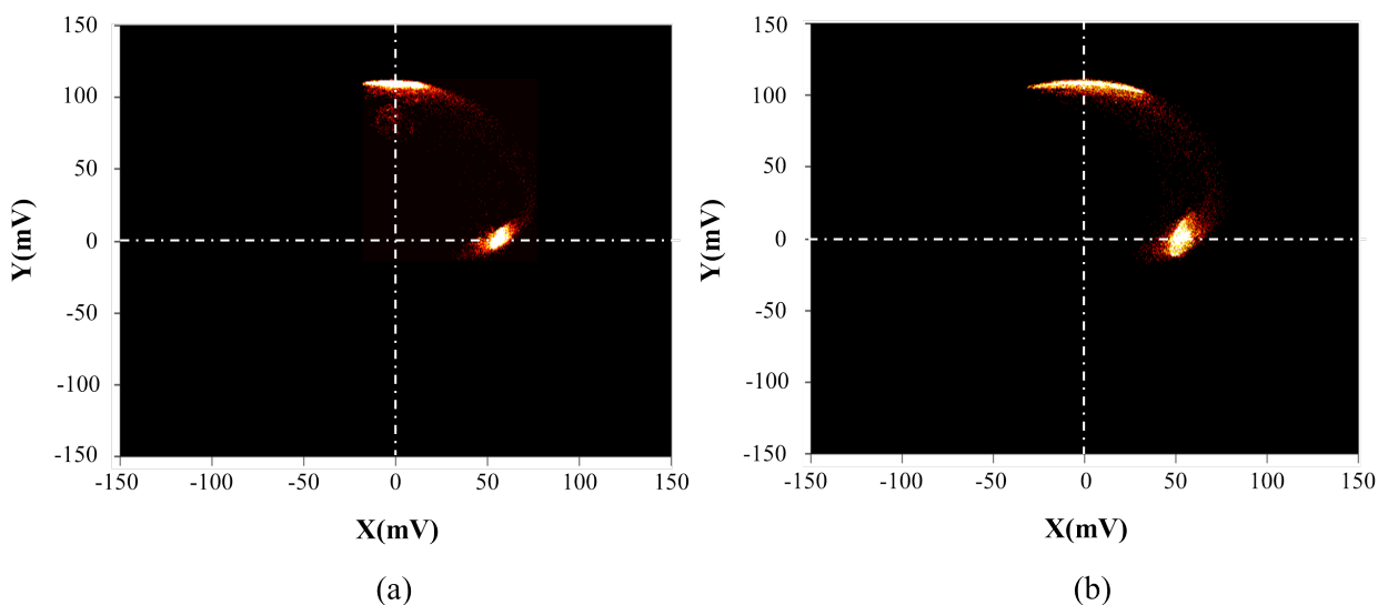
Figure 5.24: (a) Phase trajectory for stochastic resonance for an amplitude modulation of 10% (b) phase trajectory for stochastic resonance at an amplitude of modulation of 20%; with expectedly higher dispersion of the states are observed for higher modulation in amplitude.
