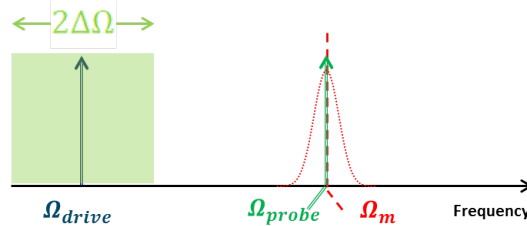
Figure 4.13: Schematic diagram of superharmonic resonance experiment: The drive frequency \Omega_{drive} is swept around \Omega_{m0}/n while at the same time the system is probed around the natural resonance of the system \Omega_{m0} .
