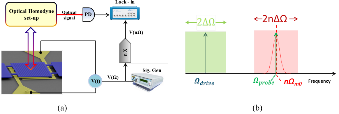
Figure 4.9: (a) Experimental set up for driving and probing the higher harmonics (b) Schematic of the probing scheme.
