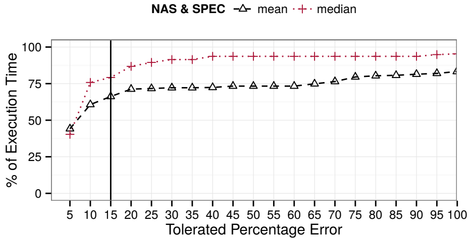
Figure 3.4: Mean and median captured execution time as a function of the tolerated replay error. the NAS and SPEC 2006 FP benchmarks. The mean is lower than the median due to the IO-intensive and short kernel benchmarks described in the validation section 5.3, which skew the distribution.
