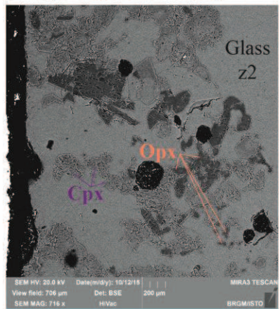
i HP10*** (T=1250°C / P=1GPa)
