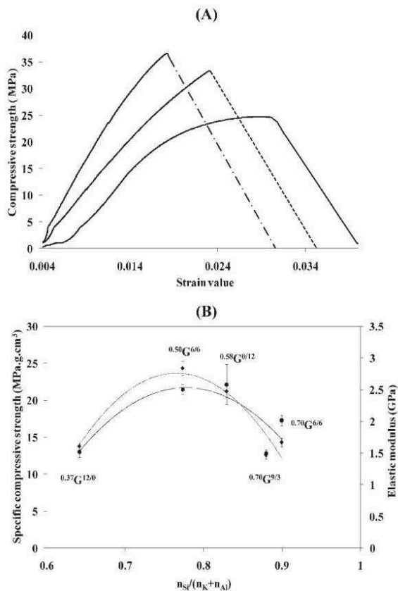
Fig. 5. (A) Compressive strength as a function of the strain value for (—) ^{0.37}G^{12/0} , (-.-) ^{0.50}G^{6/6} and (-.-.-) ^{0.58}G^{0/12} samples and (B) evolution of (●) the specific compressive strength value and the (◆) elastic modulus versus the chemical composition ( n_{Si} / (n_K + n_{Al}) ) of the different mixtures.
