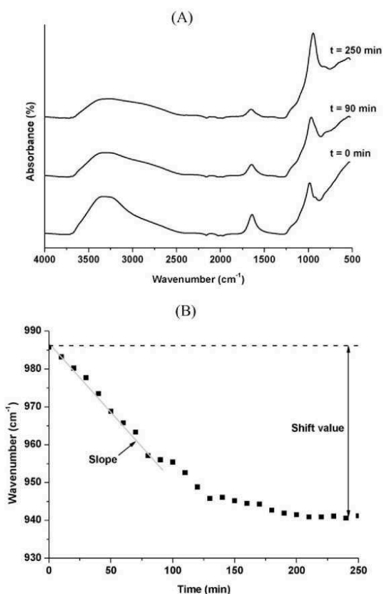
Fig. 4. In situ FTIR spectra obtained at t = 0 , t = 90 and t = 250 min for the (A) ^{12,51}\text{G}^0 and (B) \text{Q}^2 position shift and slope from IR spectra versus time for the ^{12,51}\text{G}^0 sample.
