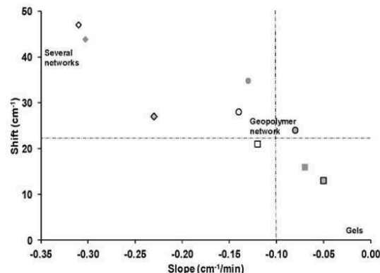
Fig. 6. Evolution of the shift versus the slope for different compositions ( \diamond ) ^{12.51}G^0 , ( \blacklozenge ) ^{12.51}G^{20} , ( \bullet ) ^{12.51}G^{520} , ( \circ ) ^{12.53}G^0 , ( \blacksquare ) ^{12.53}G^{20} , ( \blacktriangle ) ^{12.53}G^{520} , ( \square ) ^{20.51}G^0 , ( \blacksquare ) ^{20.51}G^{20} and ( \blacksquare ) ^{20.51}G^{520} samples.
