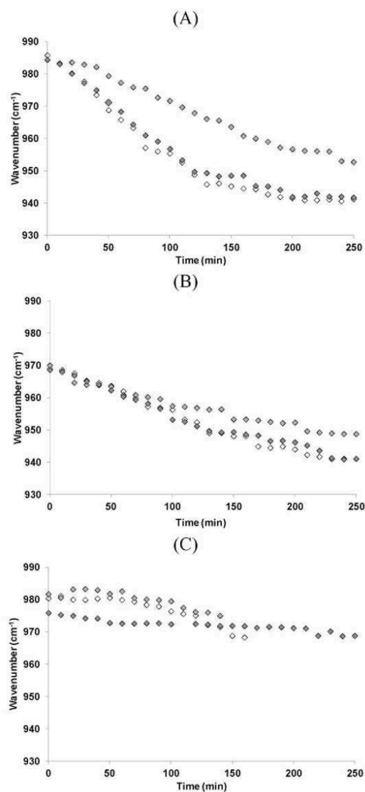
Fig. 5. Evolution of the shift of \text{Q}^2 position from FTIR spectra versus time for (A) ^{12,51}\text{G}^x , (B) ^{12,53}\text{G}^x and (C) ^{20,51}\text{G}^{5x} reactive mixtures with x = (\diamond) 0 , (\oplus) 20 and (\ominus) 520\% of crushed geopolimer.
