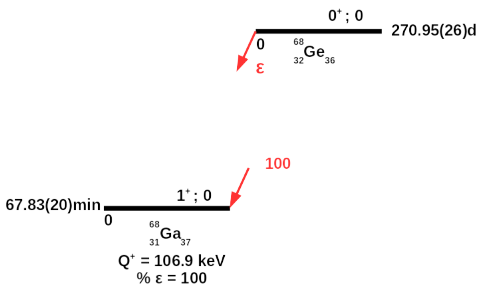
Figure A.1: The decay scheme of ^{68}\text{Ge} , which has a half life of 270 days and is 100 % produced by electronic capture going into ^{68}\text{Ga} .
