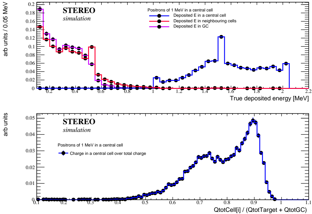
Figure 5.4: (top) Deposited energy for positrons of 1 MeV uniformly distributed in a central cell. In most cases at least one 511 keV gamma leaks to the neighboring cells or GC. (bottom) Collected charge in cell of interaction for positrons of 1 MeV. Most of the charge is collected in the same cell, while in neighboring cells a 511 keV gamma can be registered.
