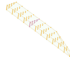
VisualPolylib visualization.
