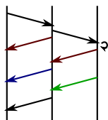
Sequence diagram
