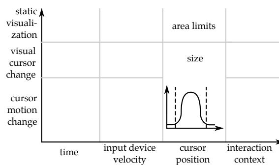
Figure 75 – "Bumps and Holes" experiment [170] in the transfer function arguments design space.
