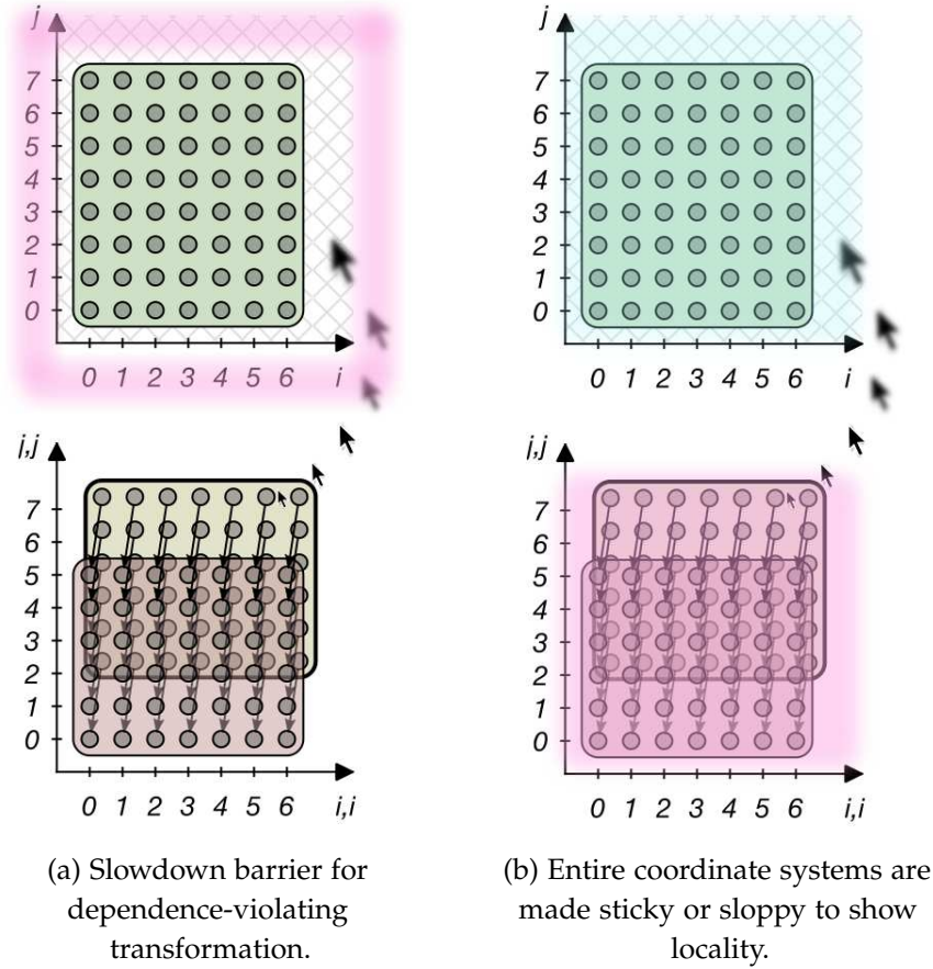
Figure 93 – C-D gain modifications in Clint for statement-level transformations: light blue overlays show cursor speedup areas, darker purple overlays show cursor slowdown areas; the target coordinate system features crossing diagonal lines in the background.
