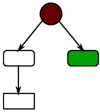
Node-link diagram
