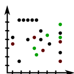
Scatter plot
