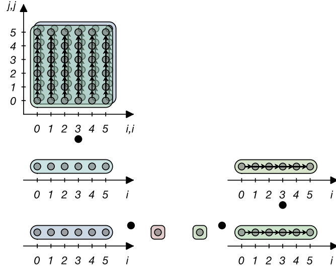
Figure 59 – The refined optimized version of the conventional beamforming radar kernel visualized with Clint
