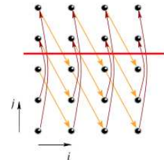
LooPo visualization.
