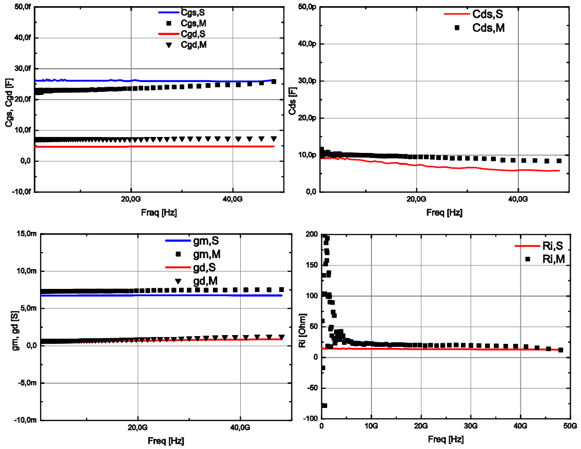
Figure 35 : The extraction of intrinsic small signal parameters of the 20μm x 0.25μm RFMOS transistor
