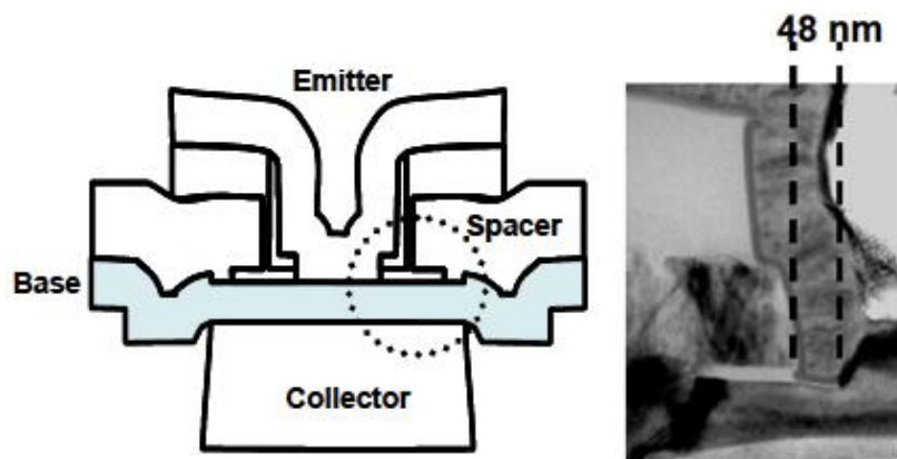
Figure 4 : Schematic cross section of the NPN device [13]
