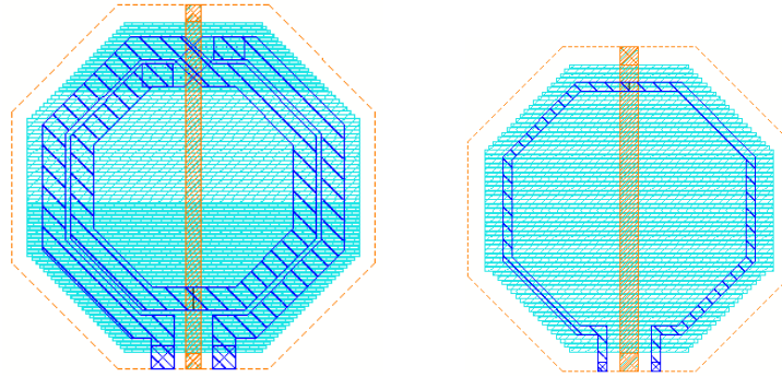
Figure 24 : Layout of the octagonal inductors with a 0.25 \mu m BiCMOS technology, two turns (left) and single-loop (right). The ground shield consists of the polysilicon bars perpendicular to the symmetry plane of the inductor
