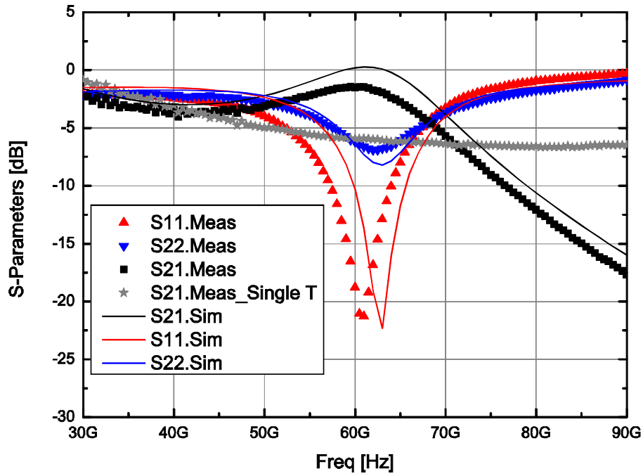
Figure 64 : Matched test structure S-parameters measured and simulated
