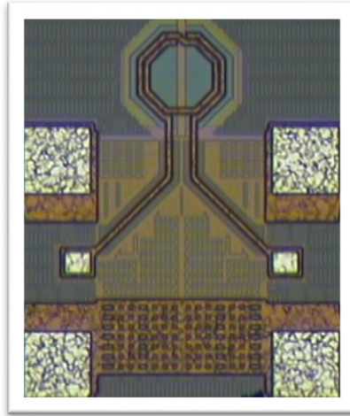
Figure 31 : Photograph of the inductor 2 in the new test structure
