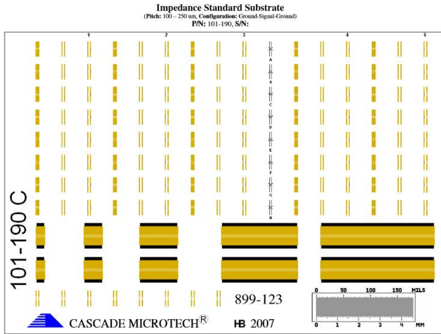
Figure 12 : Calibration substrate used for calibration
