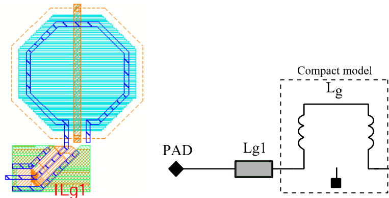
Figure 47 : Interconnection between input pad and compact model inductor. All interconnections are included in simulation
