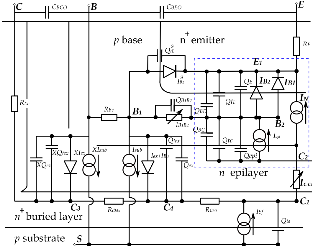
Figure 52 : The complete Mextram equivalent circuit for the vertical NPN transistor
