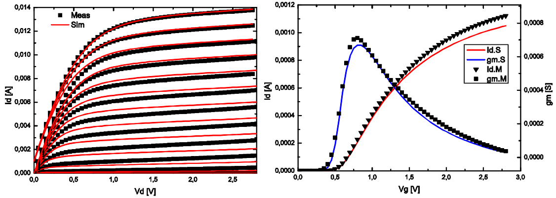
Figure 34 : Example of measured and simulated output characteristics ( I_{ds} - V_{ds} ), input characteristic ( I_{ds} - V_{gs} ), and transconductance for a 20 \times 0.25 \mu\text{m} NMOS transistor
