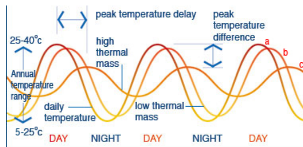
FIGURE 1.3 – Temperature variations in the use of thermal mass
