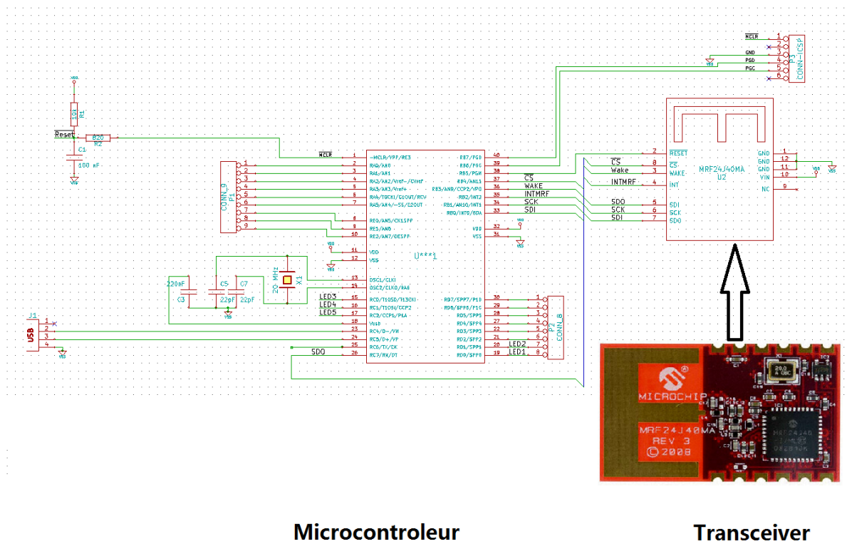
FIGURE 7.2 – WSN system design with MRF24J40MA
