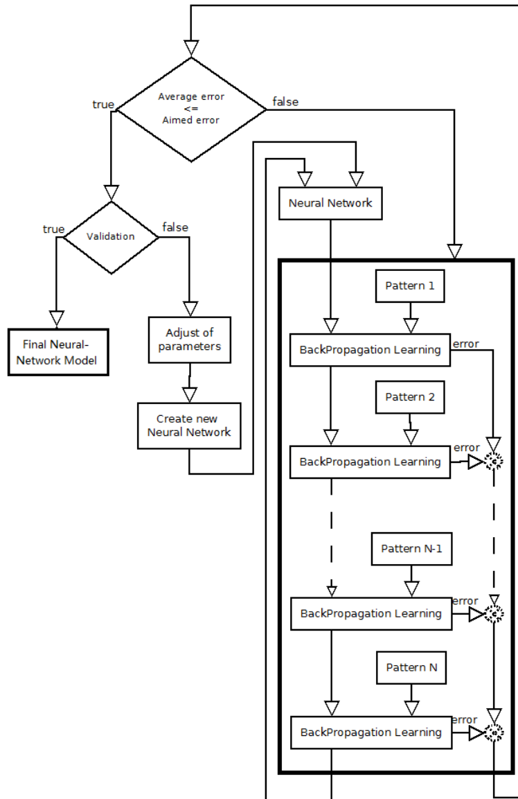
FIGURE 11.1 – Multi-Pattern Cross Training Method.
