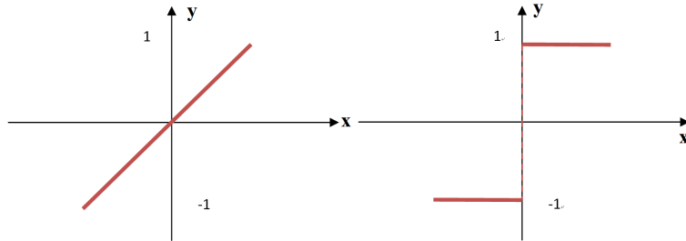
FIGURE 3.5 – Activation function
