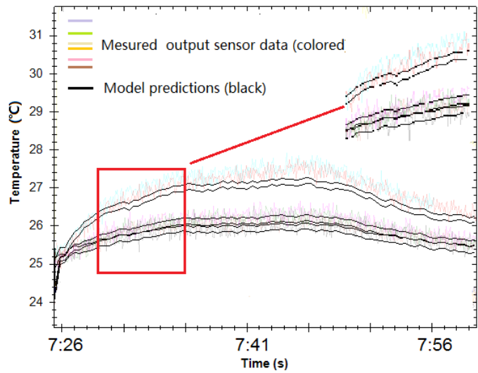
b. Model response regarding test data
