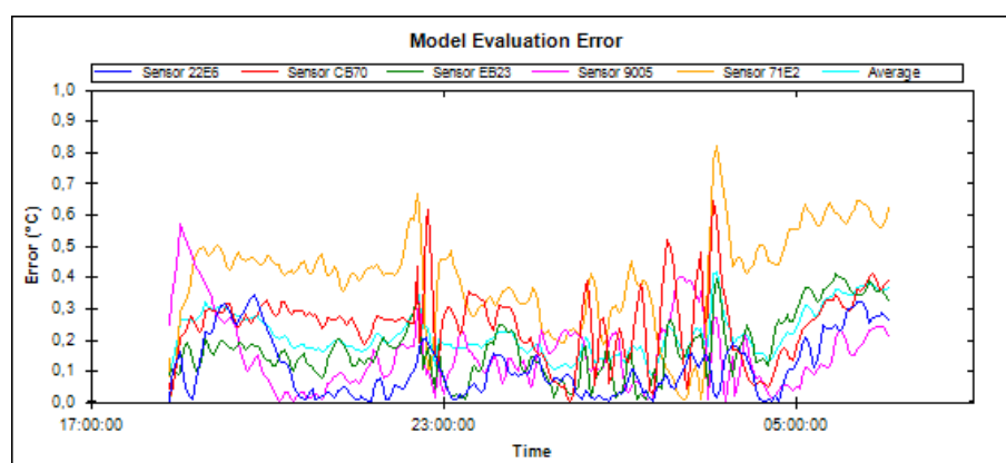
FIGURE 9.12 – Error curves of each sensor in one session ( MSE = 0,27^{\circ}C ).
