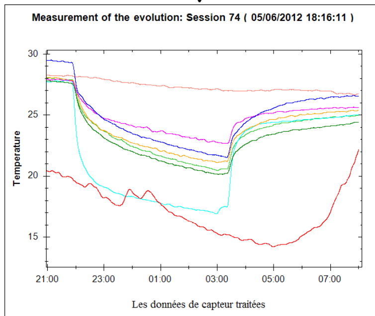
FIGURE 9.11 – The filtered sensor data
