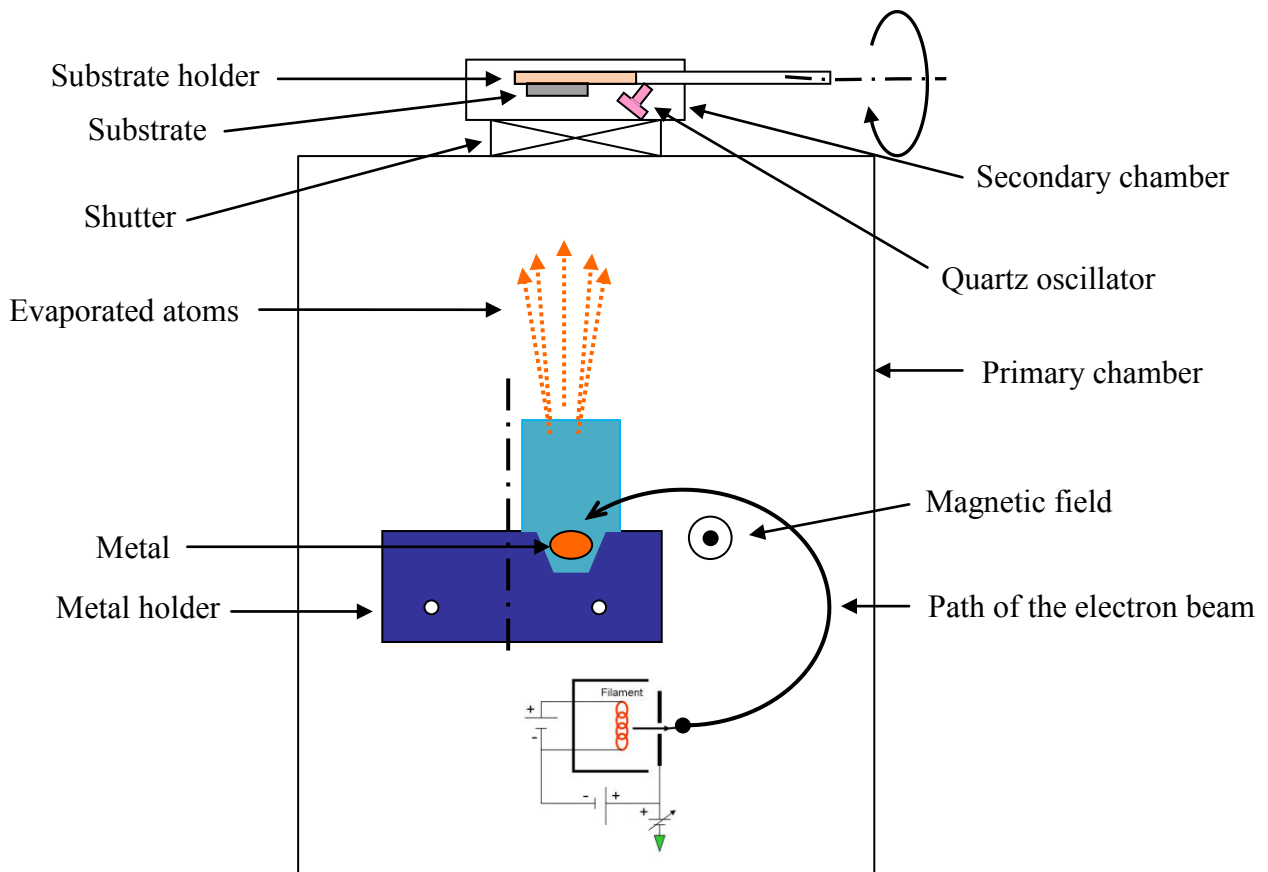
Figure 3.1. Schematic representation of the electron beam physical vapour deposition system (EBPVD). The evaporation material is held at a positive potential relative to the filament. To avoid chemical interactions between the filament and the evaporation material, the filament is kept out of sight. A magnetic field is employed to direct the electron beam from its source to the material location.
