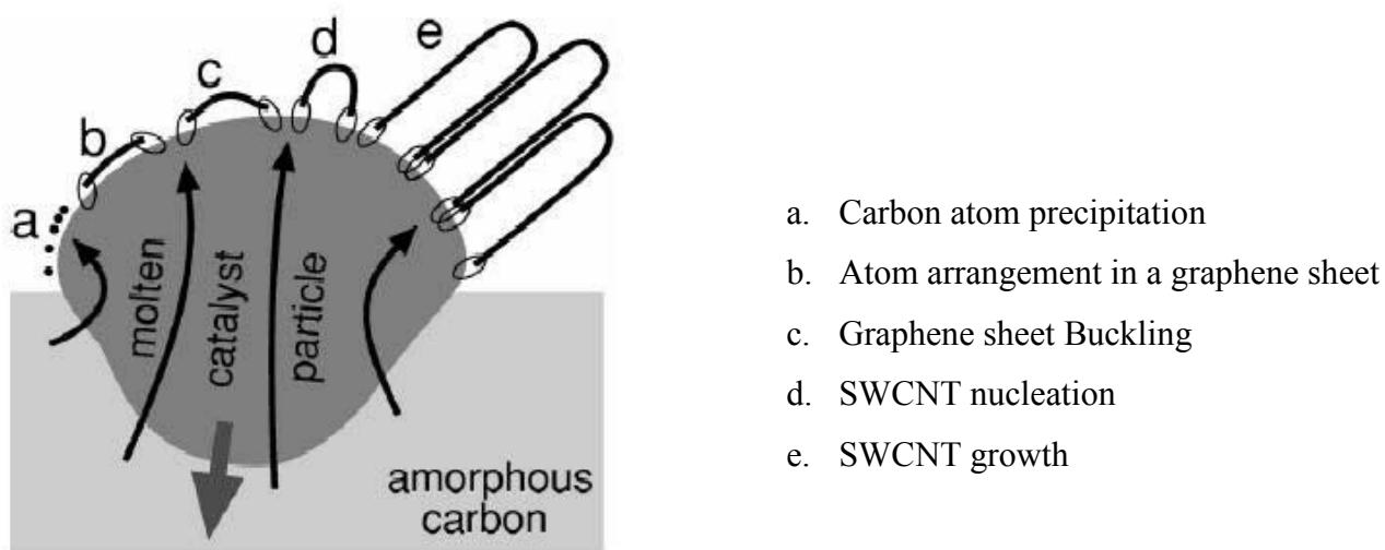
Figure 4.46. The proposed solid-liquid-solid mechanism of SWCNT nucleation and growth by dissolution-precipitation of amorphous carbon condensed at early stages of the reaction. Ellipses symbolize the overlapping metal-carbon electron orbitals.
