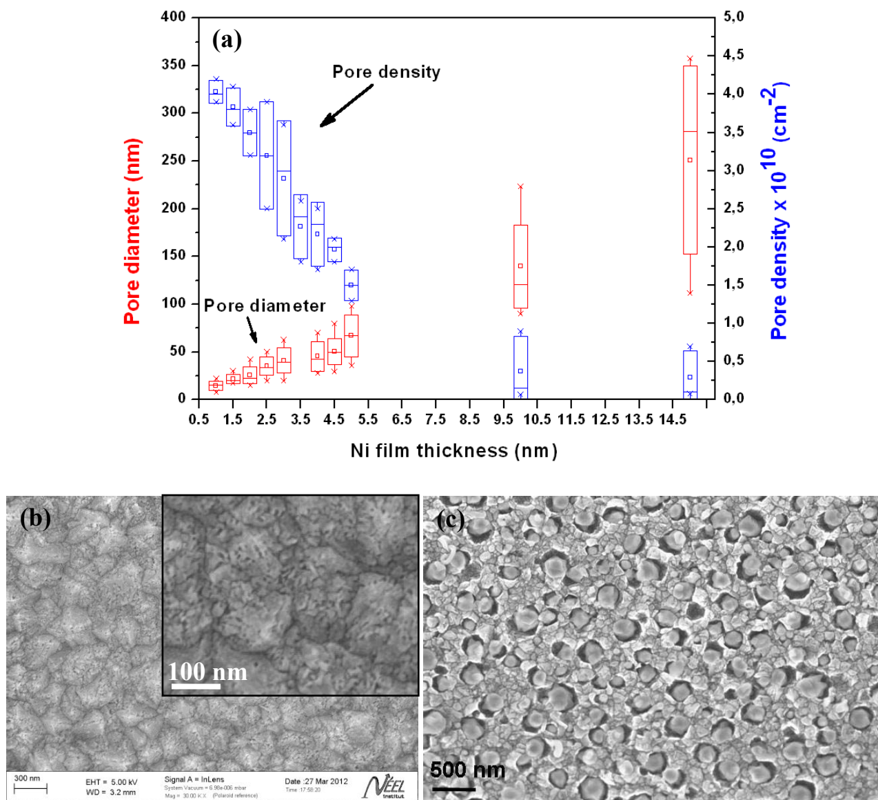
Figure 5.7. (a) Nanopore diameter and density distribution measured for nanocrystalline diamond after 10 min annealing with Ni layers of thickness of 1 to 15 nm, (850 °C, 60 Torr H 2 ). The box represents standard deviation. The band and square inside refer to median and mean respectively; minimum and maximum values are indicated by the cross. Nanopore diameter and density were estimated by analyzing the SEM images of each processed sample. (b) corresponding SEM image
