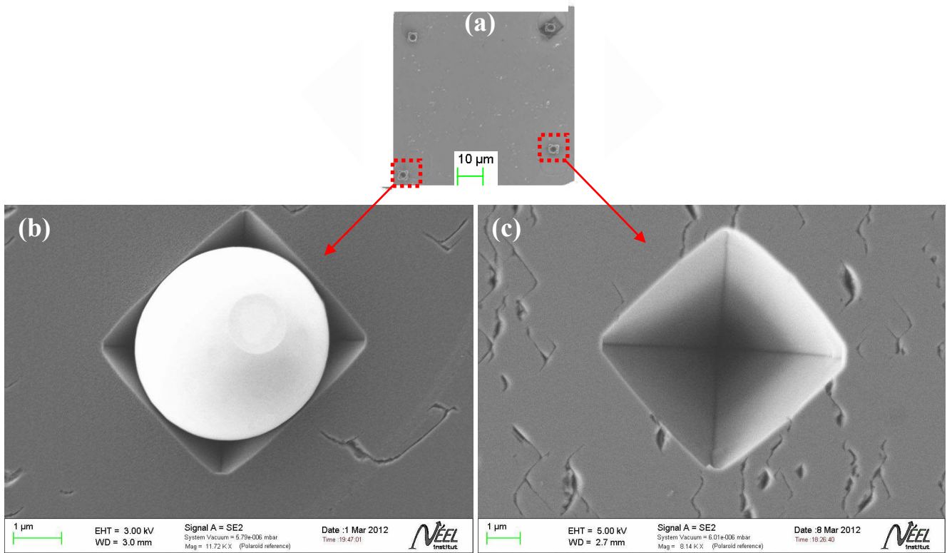
Figure 5.24. The morphology of etched microstructures in [100] -oriented single crystalline diamond after 1 hour of annealing with 200 nm patterned Pd film, (850 °C, 60 Torr); (a) low magnification SEM image showing few ordered microstructures, (b) SEM image acquired with a secondary electron image where spherically shaped particles (bright contrast) corresponds to Pd and (c) secondary electron image after Pd removal by aqua regia revealing the inverse pyramidal-shape of microstructure walled by four \{111\} planes.
