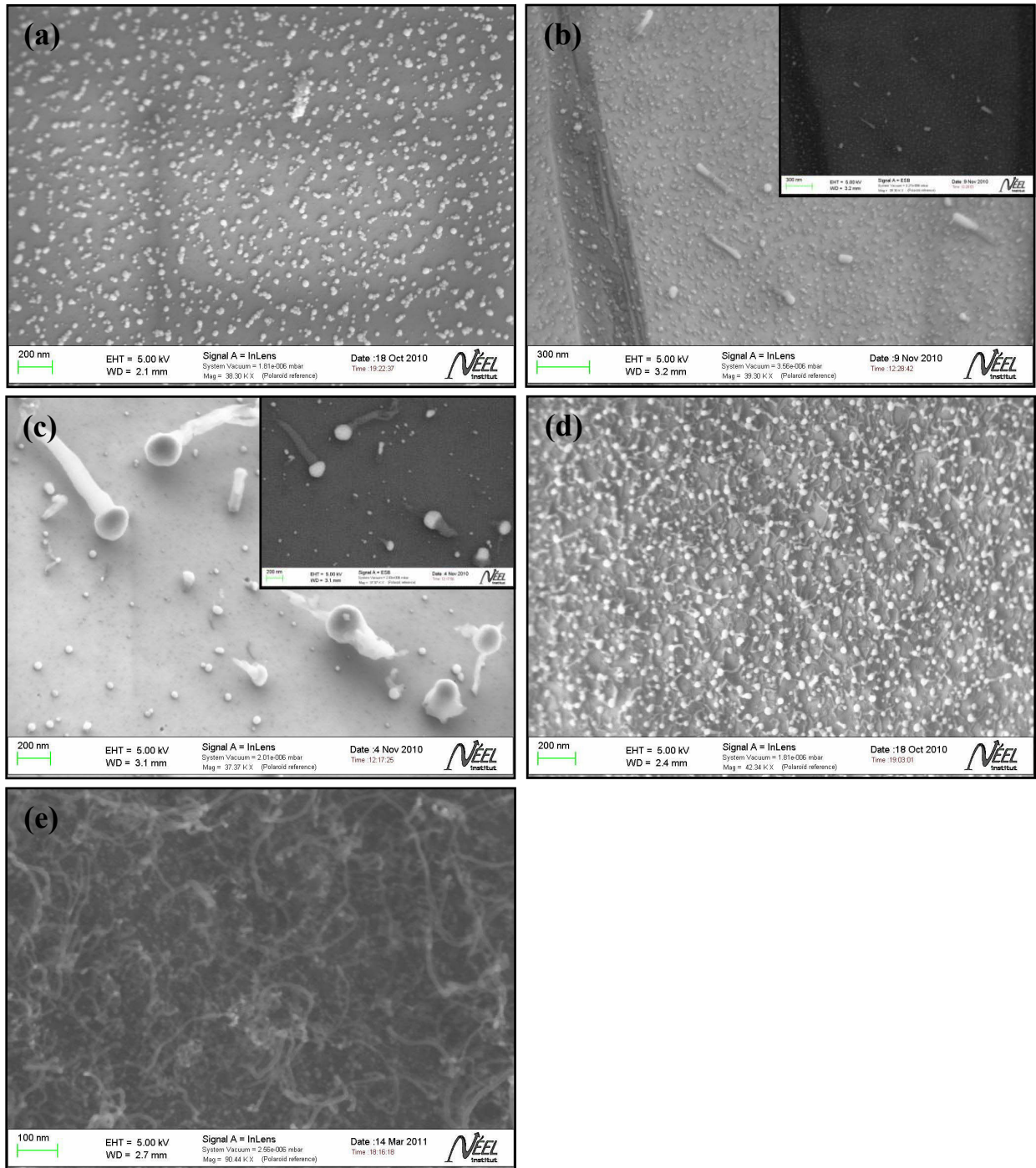
Figure 4.37. SEM images of HFCVD grown samples for 2 hours with (a) 1 vol.%, (b) 2 vol.%, (c) 3 vol.%, (d) 4 vol.% and (e) 6 vol.% CH 4 in 100 sccm H 2 , ( T_f : 2100 °C, T_s : 850 °C, P_{H_2} : 30 Torr). The insets of panels (b) and (c) are corresponding, ESB detected SEM images.
