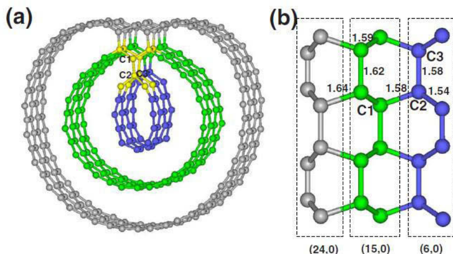
Figure 1.9. Structure resulting from intershell C-C bonding in a MWCNT according to first-principles DFT calculations. Optimized atomic configuration of MWCNT with (6, 0), (15, 0), and (24, 0) concentric inner (colored in blue), middle (colored in green), and outer (colored in gray) nanotubes, respectively, depicting intershell C-C bonding. (a) Top view along the axial direction. (b) Cross-sectional view on the symmetry plane. Blue, green, and yellow spheres denote C atoms. The yellow-colored C atoms highlight the seed unit for the nucleation of a bulk phase of hexagonal diamond (lonsdaleite). The figure is adapted from Muniz et al. 2009 .
