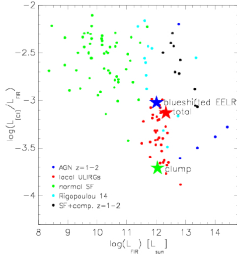
Figure 7.10: L_{\text{[CII]}}/L_{\text{FIR}} versus L_{\text{FIR}} relationship for different regions in the Garnet, compared to populations of low and high-redshift galaxies in the literature. We show the position of the blue emission line region in G045.1 (blue star), as well as the continuum source (green star) and the total source (red star), after correcting for the gravitational magnification. The external samples comprise the intermediate redshift ULIRGs of Rigopoulou et al. (2014) ( 0.2 < z < 0.8 ) and the actively star-forming or AGN-dominated galaxies of Stacey et al. (2010) ( z \sim 1 - 2 ).
