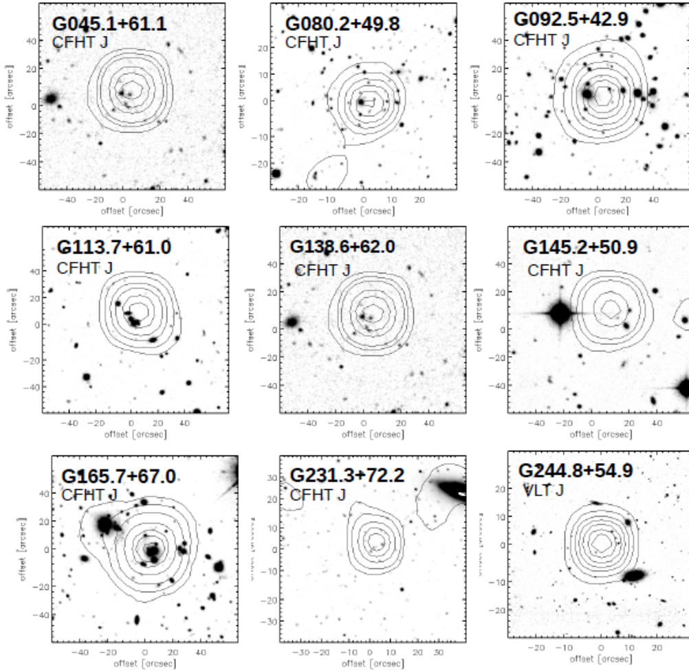
Figure 4.5: Near-infrared J-band images of the nine GEMS for which we obtained optical/NIR imaging and millimetre interferometry before 2015 (Fig.4.6). Contours show the Herschel/SPIRE morphology at 250 \mu\text{m} .
