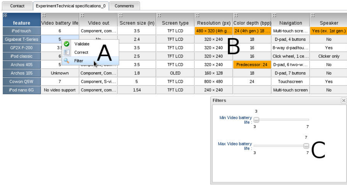
Figure 5.3: Example of a PCM Editor with Warnings and Filtering
