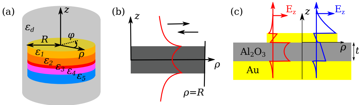
Figure 2.14 – Patch antenna model: theoretical configuration and definitions.
