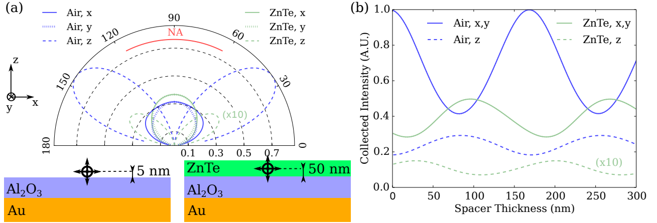
Figure 3.14 – Effect of the Al 2 O 3 spacer thickness on the properties of a radiating dipole. (a) Stacked Al 2 O 3 -Au and ZnTe-Al 2 O 3 -Au systems with the radiating x , y and z dipoles, and corresponding radiation patterns for a 250 nm thick spacer at a wavelength of 620 nm. The experimental numerical aperture NA=0.45 is indicated in red, and the legend indicates the surrounding material of the dipole and its orientation. The x and y -oriented dipoles have very similar radiation patterns in the x-z plane, with a well-centred emission lobe towards the z axis. (b) Integrated intensity in the experimental NA for each configuration as a function of the Al 2 O 3 thickness. The lines corresponding to the y dipole are superimposed with the x dipole ones. For both panels, note that the (ZnTe, z ) curve has been multiplied by 10 for visibility. From these simulations, we can deduce that the optimum spacer thickness for a CdTe QD in a ZnTe NW is around 250 nm.
