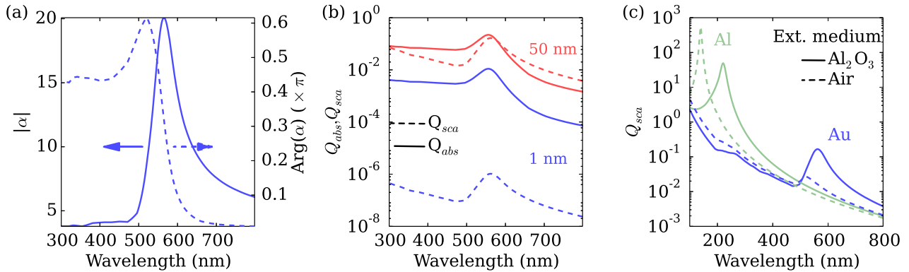
Figure 1.10 – LSPR in the quasi-static approximation.
