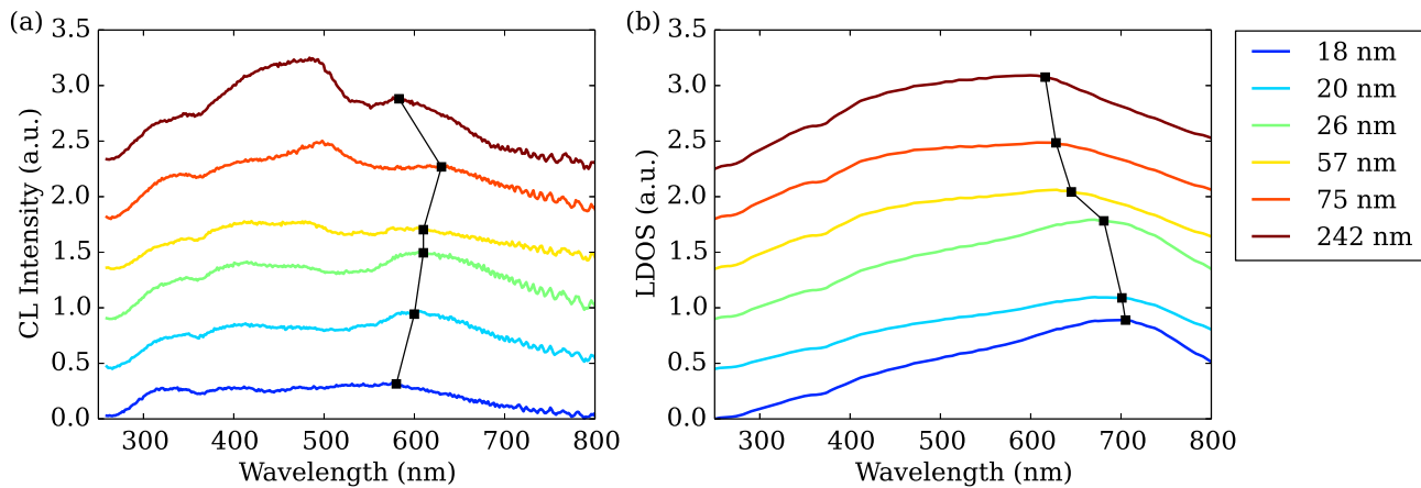
Figure 2.10 – CL and plasmonic LDOS of Au- \text{Al}_2\text{O}_3 -Au structures.
