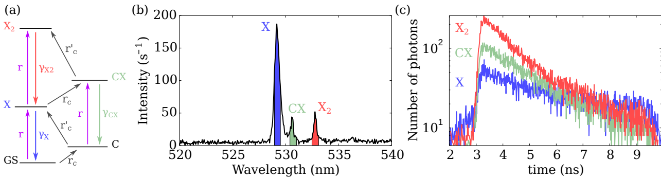
Figure 3.10 – Principle of time-resolved spectroscopy.
