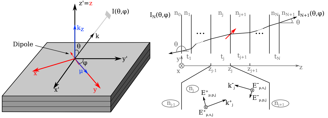
Figure 3.13 – Radiating dipole inside a multilayer system.
