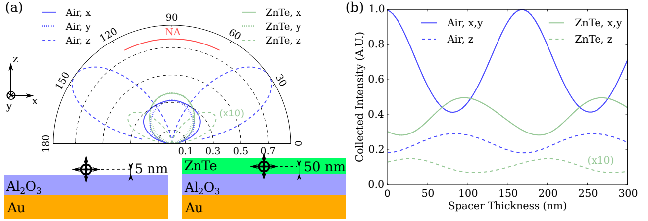
Figure 3.14 – Effect of the Al 2 O 3 spacer thickness on the properties of a radiating dipole. (a) Stacked Al 2 O 3 -Au and ZnTe-Al 2 O 3 -Au systems with the radiating x , y and z dipoles, and corresponding radiation patterns for a 250 nm thick spacer at a wavelength of 620 nm. The experimental numerical aperture NA=0.45 is indicated in red, and the legend indicates the surrounding material of the dipole and its orientation. The x and y -oriented dipoles have very similar radiation patterns in the x-z plane, with a well-centred emission lobe towards the z axis. (b) Integrated intensity in the experimental NA for each configuration as a function of the Al 2 O 3 thickness. The lines corresponding to the y dipole are superimposed with the x dipole ones. For both panels, note that the (ZnTe, z ) curve has been multiplied by 10 for visibility. From these simulations, we can deduce that the optimum spacer thickness for a CdTe QD in a ZnTe NW is around 250 nm.
