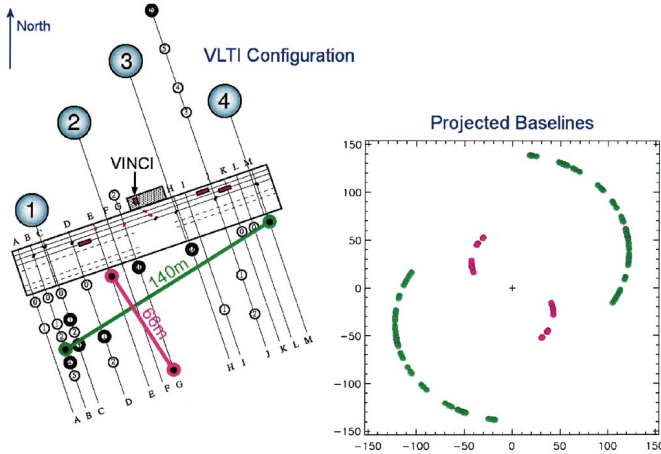
Fig. 1. VLTI ground baselines for Achernar observations and their corresponding projections onto the sky at different observing times. Left: Aerial view of VLTI ground baselines for the two pairs of 40 cm siderostats used for Achernar observations. Color magenta represents the 66 m (E0-G1; azimuth 147^\circ , counted from North to East) and green the 140 m (B3-M0; 58^\circ ). Right: Corresponding baseline projections onto the sky ( B_{\text{proj}} ) as seen from the star. Note the very efficient Earth-rotation synthesis resulting in a nearly complete coverage in azimuth angles.
