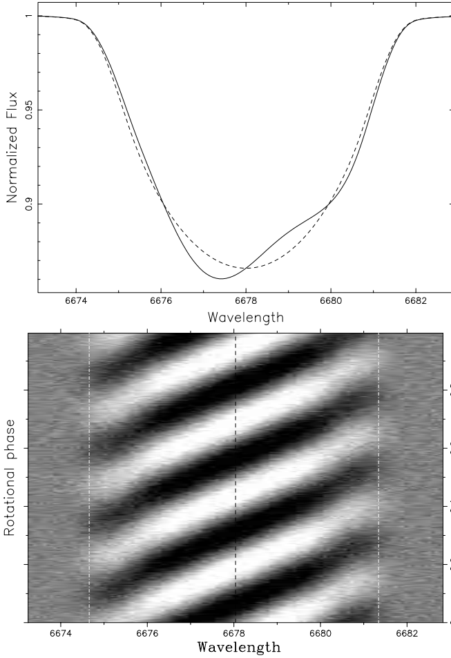
Fig. 3. Synthetic normalized flux in the He I spectral line. Top: the spectrum calculated for \Phi = 0 , using the model from Fig. 2 (solid line). The dashed line represents the spectrum corresponding to the homogeneous stellar surface. Bottom: dynamic spectrum of residuals (immaculate star profiles are subtracted from perturbed profiles) evenly spread throughout the rotational cycle. Artificial Gaussian noise ( 1/\sigma = 1000 ) is added.
