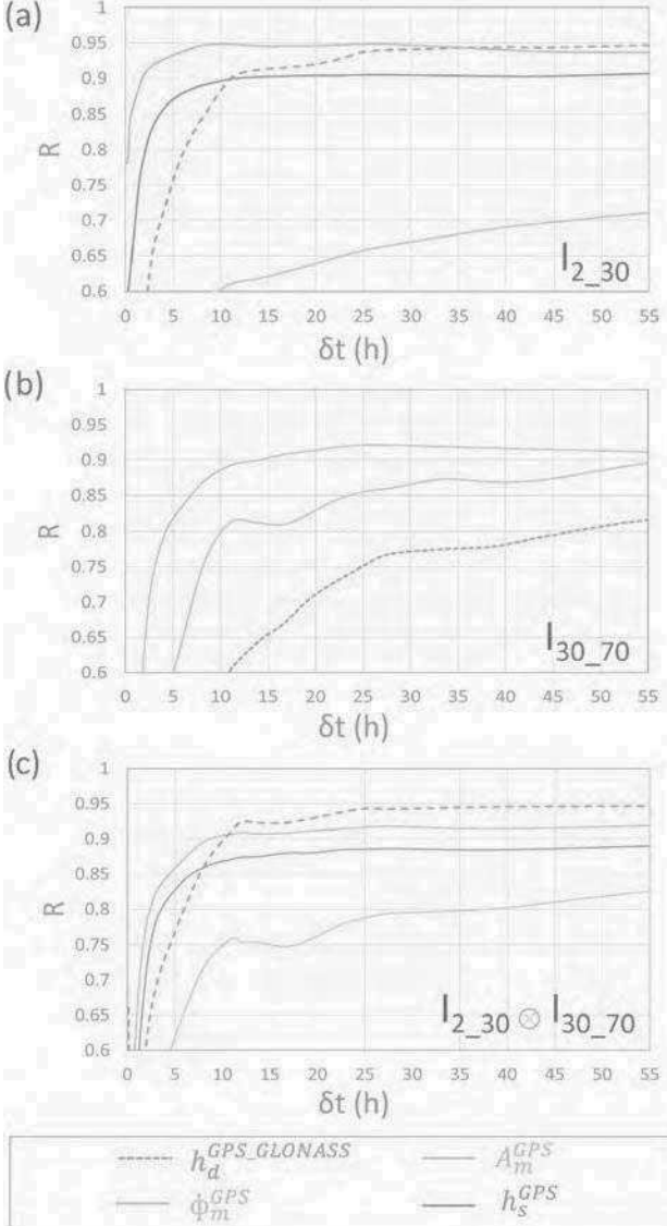
Fig. 9. (Absolute) Linear correlation coefficient R between A_m^{GPS} , \phi_m^{GPS} , h_s^{GPS} , and h_d^{GPS\_GLONASS} with P_{2\text{ cm}} , considering I_{2\_30} (a), I_{30\_70} (b) and the combination of both I_{2\_30} \otimes I_{30\_70} (c). R coefficient is below 0.4 for h_s^{GPS} .
