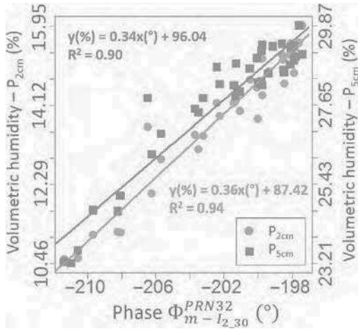
Fig. 8. Scatter plot of \phi^{PRN32}_{m-I_{2,30}} time series and P_{2cm} and P_{5cm} .
