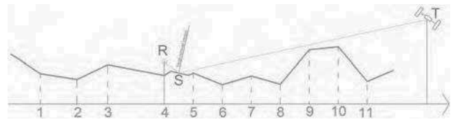
Figure 5. Determination of the specular reflection point integrating a DEM. S : specular reflection point position. R : receiver position. T : transmitter/satellite position. A dichotomous process is applied for each topographic segment of the DEM to find if there is a point where the bisecting angle (equal to the sum of the anti-incident and scattering vectors) is colinear with the local normal vector.
