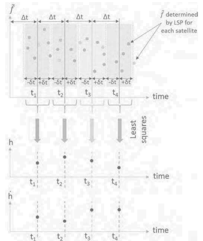
Fig. 3. Principle of the Least Squares inversion Method used to determine h and \dot{h} based on LSP estimates of f . For reasons of clarity, overlapping was not represented in this figure, even if in our case \delta t > \Delta t .
