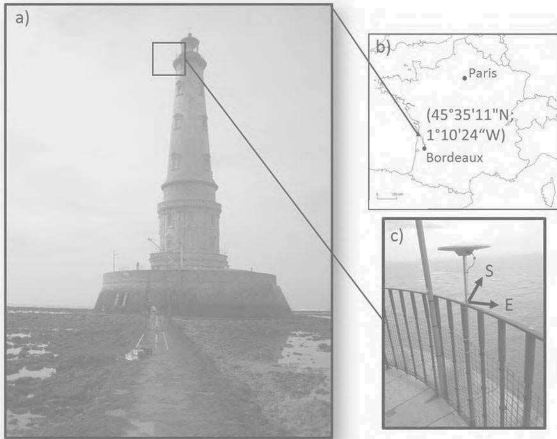
Fig. 4. Trimble Zephyr Geodetic 2 antenna with Trimble NetR9 receiver on top of Cordouan lighthouse at approx. 60 m above sea level (a). The Cordouan lighthouse (45°35'11"N; 1°10'24"W) is located at the mouth of the Gironde estuary in the South West of France (b). A Trimble NetR9 receiver with a Zephyr Geodetic 2 antenna were installed close to the top of the lighthouse (c).
