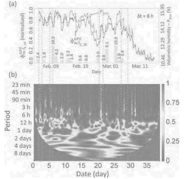
Fig. 10. (a) Evolution of \phi_{m-I_{2\_30}}^{GPS}(t) and P_{2\text{ cm}} . Linear correlation coefficient is 0.95. Blue bars are the rain events (in mm). (b) Wavelet cross correlation map: P_{2\text{ cm}} VS \phi_{m-I_{2\_30}}^{GPS} . Abscissa is the day over the 1.5-month period of measurement and ordinate is the period under analysis. Cross wavelet power is in units of normalized variance for each period.
