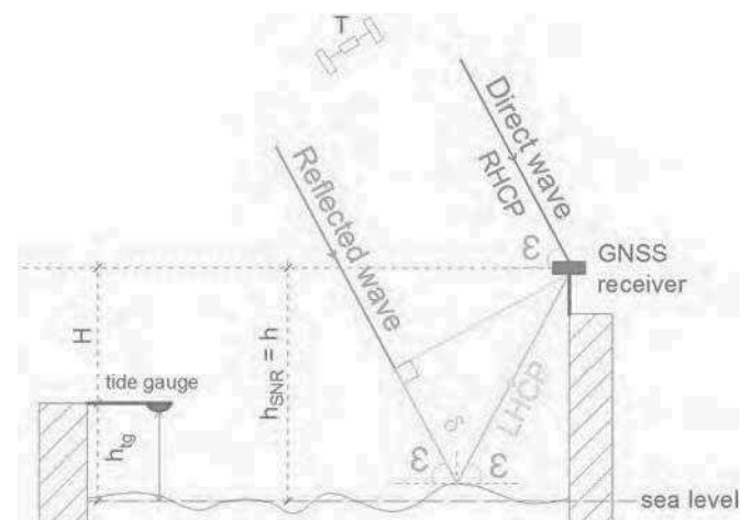
Fig. 1. Principle of GNSS tide gauge using a single GNSS antenna. \epsilon : satellite elevation angle, \delta : additional path covered by the reflected way (green line). (For interpretation of the references to color in this figure legend, the reader is referred to the web version of this article.)
