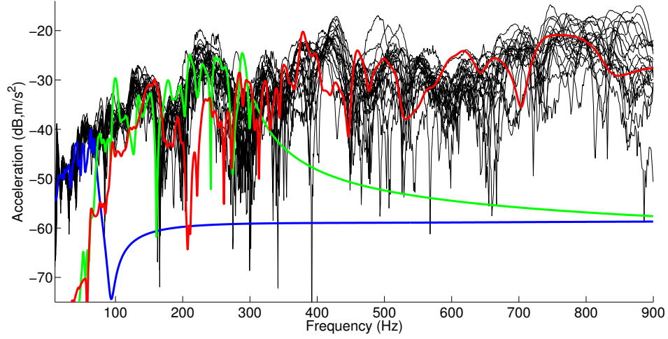
Figure 5.27: Observation 2: experimental FRF measurements performed on the PSA cars of the same type [119] (black lines), deterministic FRF using the scale- \mathcal{L} ROM (blue line), deterministic FRF using the scale- \mathcal{M} ROM (green line), and deterministic FRF using the scale- \mathcal{H} ROM (red line).
