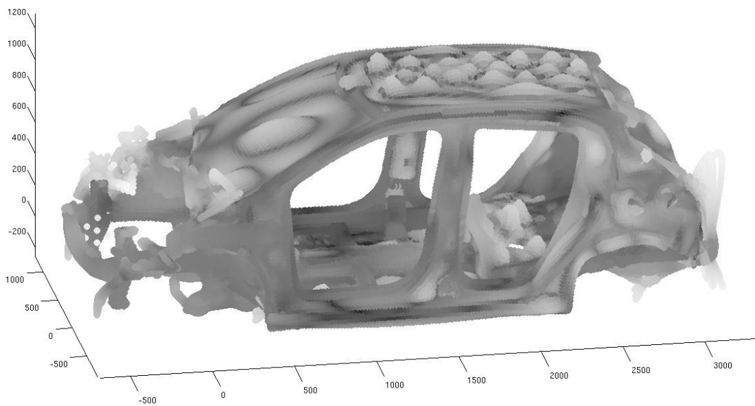
Figure 1.4: Mode shape of a regular low-frequency elastic mode of a car body structure (eigenfrequency 72 Hz).
