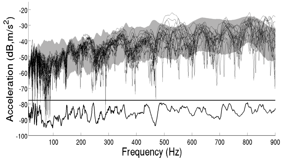
Figure 5.20: Observation 1: experimental FRF measurements performed on the PSA cars of the same type [119] (black lines), random FRF using the identified ML-SROM (gray region), and OVL function (black line underneath).
