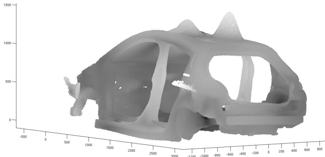
Figure 1.4: Mode shape of a regular low-frequency elastic mode of a car body structure (eigenfrequency 72 Hz).
