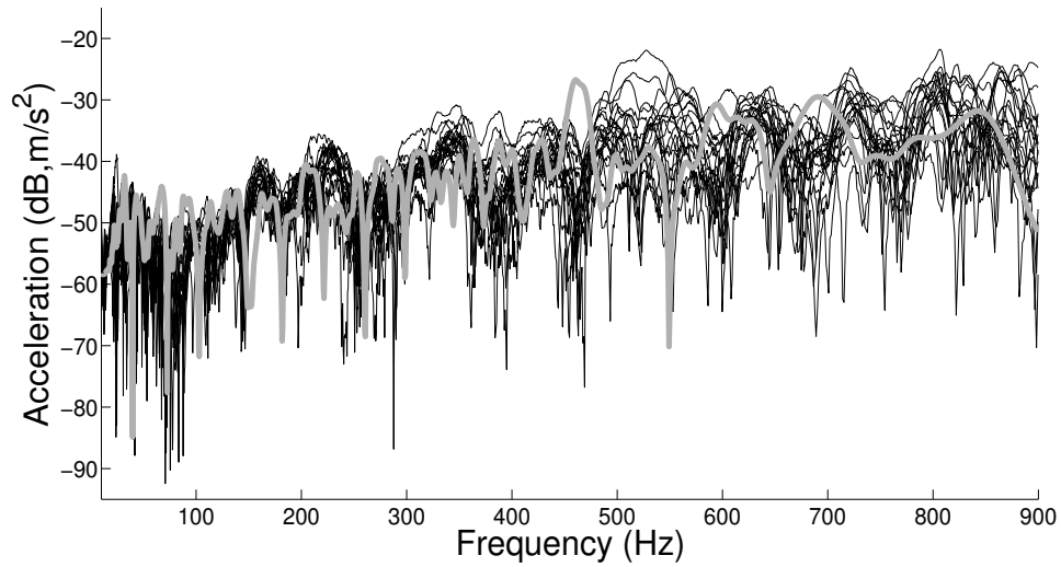
Figure 5.6: Observation 1: experimental FRF measurements performed on the PSA cars of the same type [119] (black lines), deterministic FRF using the C-NROM (gray line).
