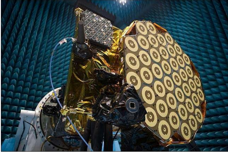
FIGURE 1.9: Earth-Facing Panel of GIOVE-B showing the navigation antenna and the LRR panel.
