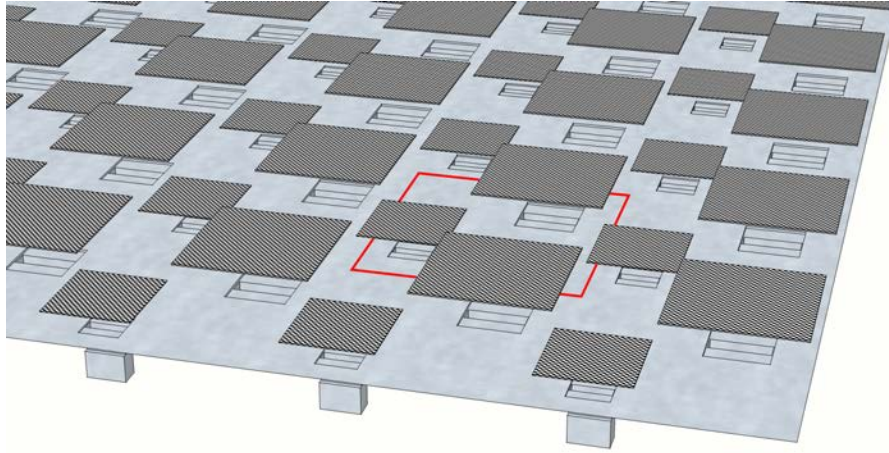
FIGURE 4.25: Sample of the dual-band chessboard array (unit cell in red).
