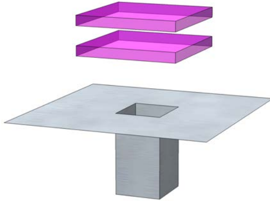
FIGURE 4.15: Patch-superstrate antenna.
