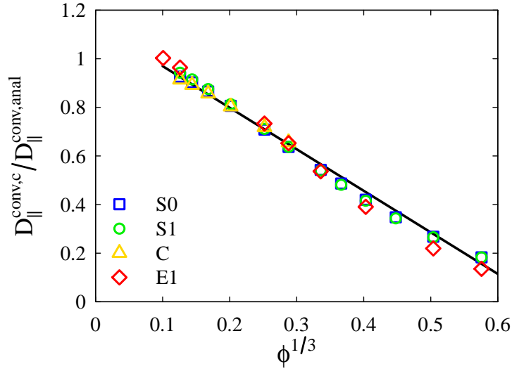
Figure 3.8 Contribution of the continuous phase D_{\parallel}^{\text{conv,c}} as a function of volume fraction for ordered arrays at Pe = 10^3 . D_{\parallel}^{\text{conv,anal}} is the asymptotic solution given by (3.41). The slope of the black line is -1.71. The colors and symbols correspond to the different flow regimes listed in table 3.1.
