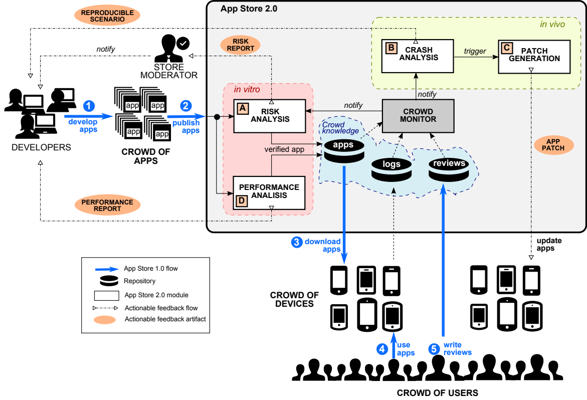
Fig. 3.5 APP STORE 2.0 workflow.
