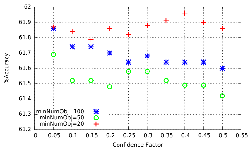
Fig. 7.3 Evaluation of the accuracy of the permission checkers.
