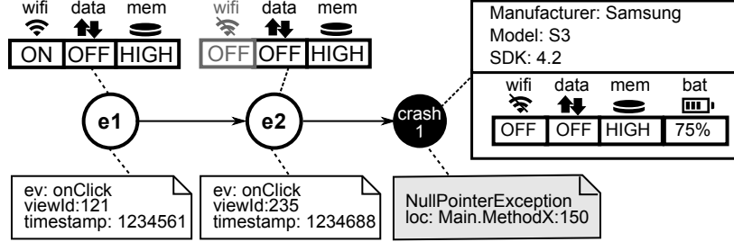
Fig. 4.5 Example of a crowdsourced crash trace.
