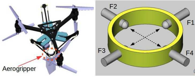
Fig. 1: Aerial grasping system (AGS): [left] AGS with cargo [right] Aerogripper scheme
