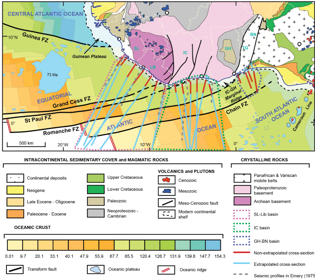
Figure 5-1 Simplified onshore geologic map and oceanic crust ages of study zone (modified from Choubert and Faure-Muret, (1988)). Location of non-extrapolated and extrapolated cross-section are indicated, as well as used seismic profiles from Emery (1975). SL: Sierra Leone, LB: Liberia, IC: Ivory Coast, GH: Ghana, TG: Togo, BN: Benin.
