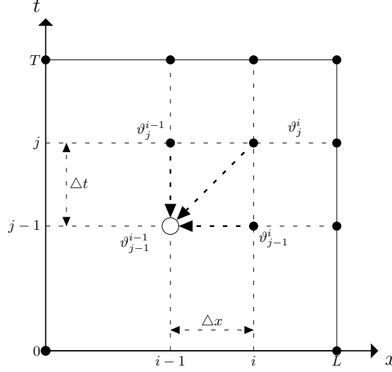
Figure II.3: Stencil of backward Preissmann scheme
