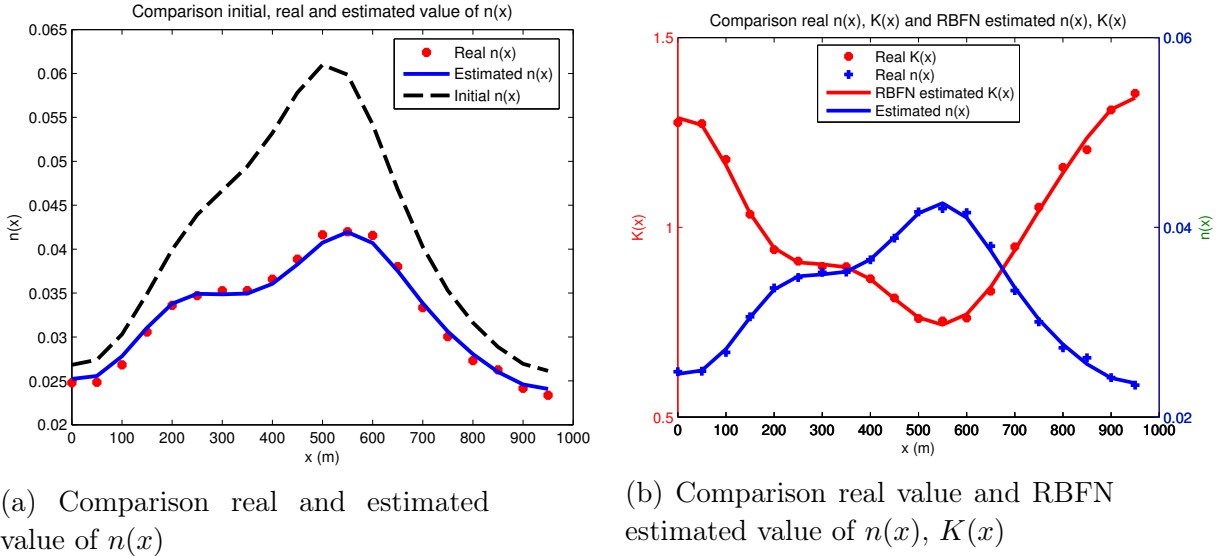
Figure III.16: Estimation results of distributed Manning coefficient in overland flow (II).
