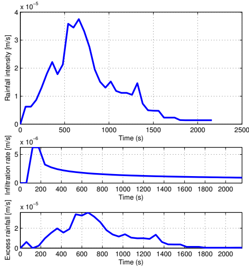
(a) Rainfall rate, soil moisture, infiltration rate, excess rainfall rate on 2012/08/03
