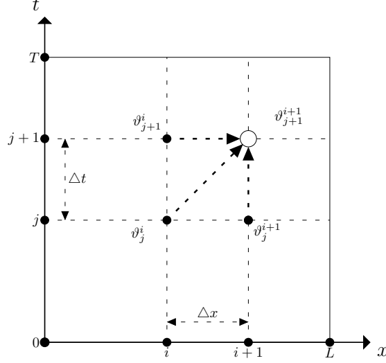
Figure II.2: Stencil of forward Preissmann scheme
