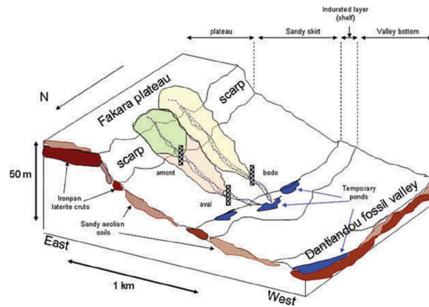
Figure III.22: Overview of Tondi Kiboro basins.
