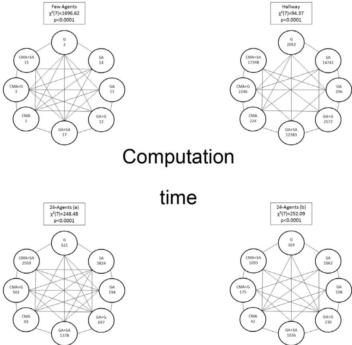
Figure A.5 – Statistical results of the Friedman’s Anova and Post-Hoc Wilcoxon signed rank tests on the computation time depending on the optimization algorithm. Mean values (s) are reported for each algorithm. Friedman’s Anova showed an influence of the optimization algorithm on the computation time for each type of data (Few Agents, Hallway, 24-Agents (a), 24-Agents (b)). Significant differences between algorithms are represented through a line ( p < 0.0018 ).
