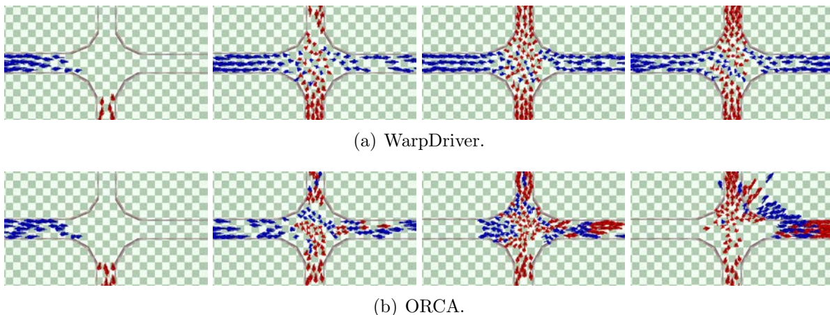
Figure 4.6 – Crossing example: two flows of agents in corridors cross at a right angle (red ones going to the top and blue ones going to the right) simulated by WarpDriver (top) and ORCA (bottom).
