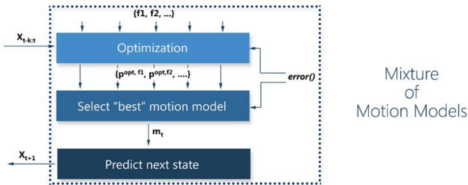
Figure 5.13 – Our parameter optimization algorithm used in Figure 5.12. Based on the error metric, we compute optimal parameters for each motion model. The best motion model (from RVO2, Social Forces or Boids) is used for trajectory extraction and to predict the next state.
