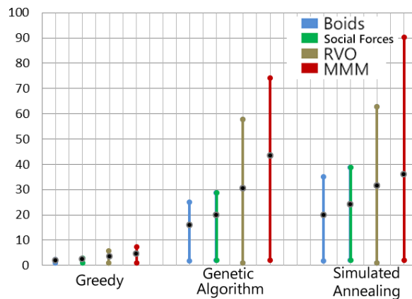
Figure 5.15 – This graph shows the time taken for each computation of every set of optimal parameters corresponding to each motion model. MMM is our approach. Time computed is in milliseconds. Each graph is a range of the scores (minimum and maximum) and the black dot is the mean score. We compute the score from the normalized error metric.
