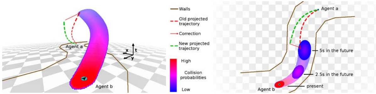
Figure 4.3 – Illustration of collision avoidance between two agents a and b on a curved path. On the left is the full 3D representation (space and time) of collision probabilities; on the right is a simplified 2D view. The color gradient represents a 's probability of collision with b , as perceived by a . The red dotted line represents a 's initial projected trajectory . The green dotted line represents a 's final, corrected, projected trajectory (exaggerated). The red line in between both dotted ones represents the correction agent a will perform (exaggerated for illustration). Note that thanks to Warp Operators , the projected trajectory is a curve instead of a straight line.
