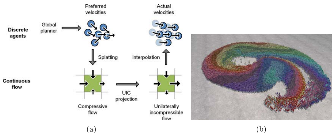
Figure 2.15 – Algorithm from [NGCL09]. (a) Workflow overview. (b) Resulting crowd.
