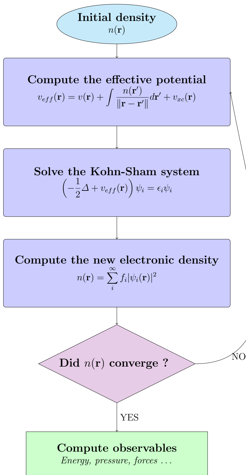
Figure 3.1: Numerical procedure used to find the electronic density for a given position of the nucleus, and hence a given v(\mathbf{r}) . The loop is repeated until the density has converged to a given convergence parameter, and then the output quantities are computed.
