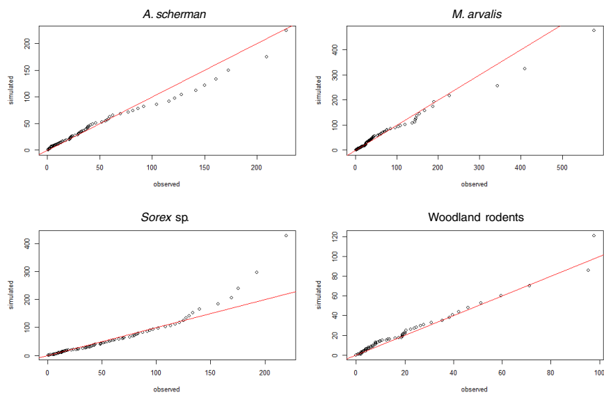
Fig. 2.9: QQplots for H3.3 model in the T. alba system. Observed and simulated data quantiles are compared for (a) A. scherman , (b) M. arvalis , (c) Sorex sp. and (d) woodland rodents.
