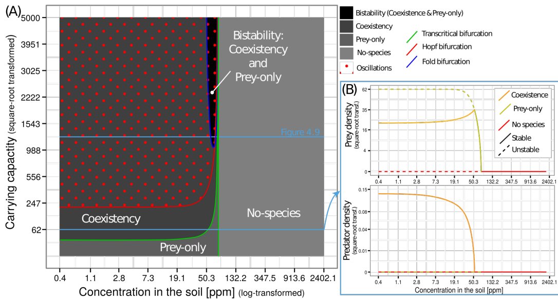
Fig. 4.10: (A) 2D-Bifurcation diagram illustrating smoothly changes and tipping points in the null model (prey concentration is equal to soil concentration C_x = C_s ). This diagram results from 500 1D-bifurcation diagram along a range of carrying capacity K \in [0, 5000] . (B) 1D-Bifurcation diagram showing a continuous change in ecosystem when the concentration in the soil increase.
