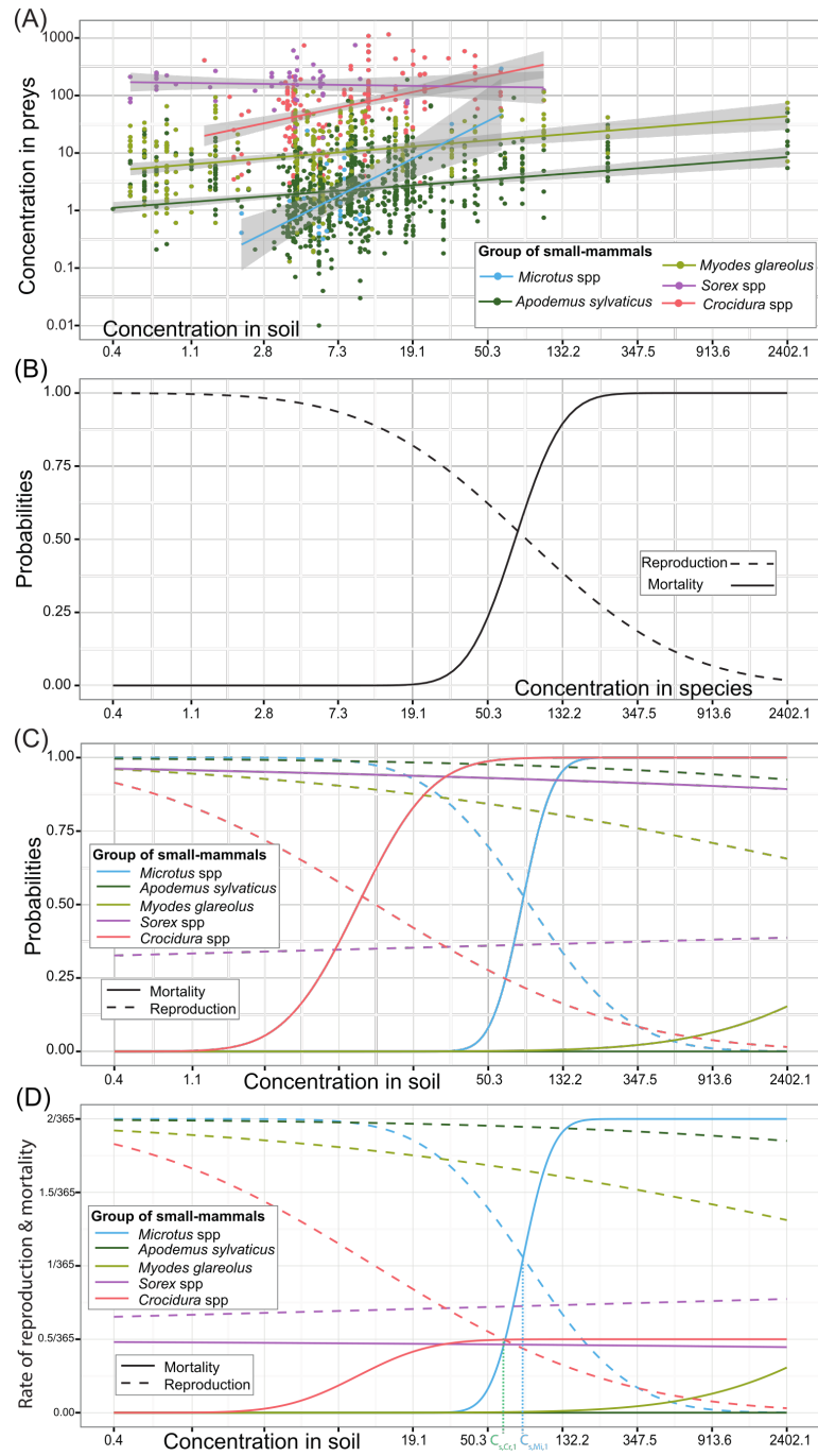
Fig. 4.8: (A) Log-log linear model with 95% credible interval from data from Metaleurop. Whole body concentration in fresh weight and concentration in soil (dry weight). Equation in Table 4.1. (B) Log-normal probabilities of reproduction and mortality for prey depending on the concentration in the species individuals. (C) Log-normal probabilities of reproduction and mortality depending on the concentration in the soil. We use same parametrization than in graph A. (D) Rate of reproduction with r = 2/365 \text{ day}^{-1} , and rate of mortality with m_{Mi,Ap,My} = 2/365 (maximal reproduction rate r ) and m_{Cr,So} = 0.5/365 (1/4 of maximal reproduction rate to have reproduction greater than mortality at C_s = 0 for Sorex spp ).
