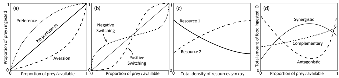
Fig. 2.4: Graphical illustration of predator's change in preference properties. (a) Preference: the solid line indicates no-preference (equal representation in diet and environment). A preference (dotted line) is an over-representation of the item in the diet, conversely, aversion (dashed line) is an under-representation of the item in the diet. (b) Switching: the dashed line is positive switching where the proportion of prey eaten is under-represented compared to prey availability until a switching point where the prey switches to being over-represented in the diet, and dotted line is a negative switching. (c) Rank switching: the rank of species in the diet changes with an increase of the total amount of prey. (d) Overall feeding isocline: total ingestion of two prey, \Theta(x_1, x_2) , depending on their relative proportion x_1/(x_1 + x_2) , with a constant sum x_1 + x_2 .
