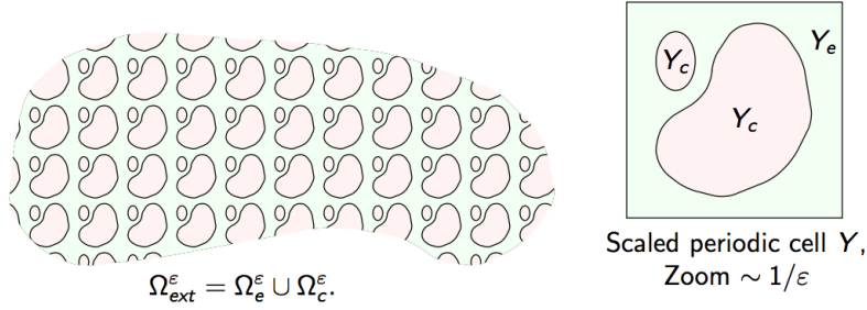
Figure 4.1 – Illustration of a periodic domain and the periodicity box Y .
