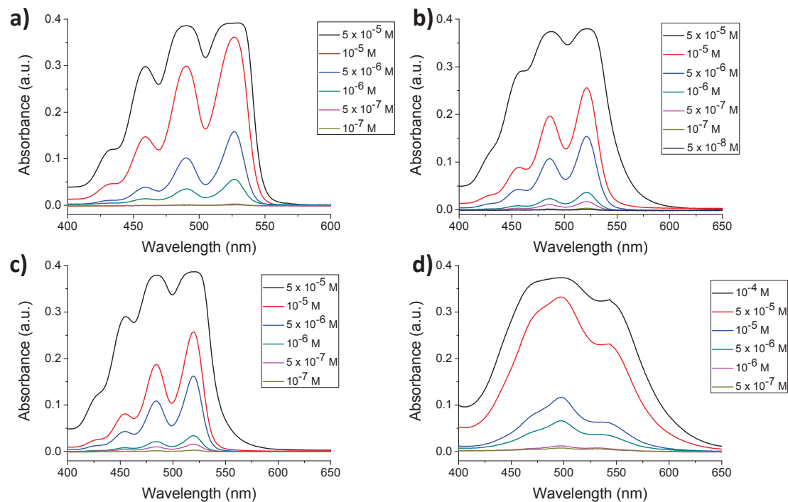
Figure 122 | a) UV-Vis spectra of a CDCl 3 solution of PBI-OPEG 7 with concentrations ranging from 10 -7 (light brown) up to 5 × 10 -5 mol/L (black); b) UV-Vis spectra of a CD 3 OD solution of PBI-OPEG 7 with concentrations ranging from 5 × 10 -8 (dark blue) up to 5 × 10 -5 mol/L (black); c) UV-Vis spectra of a CD 3 CN solution of PBI-OPEG 7 with concentrations ranging from 10 -7 (light brown) up to 5 × 10 -5 mol/L (black); d) UV-Vis spectra of a D 2 O solution of PBI-OPEG 7 with concentrations ranging from 5 × 10 -7 (light brown) up to 10 -4 mol/L (black).
