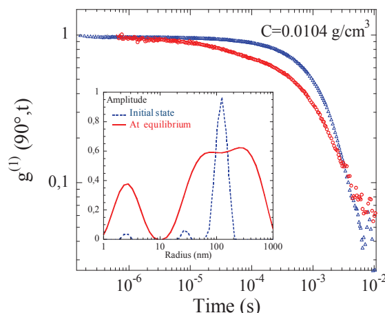
Figure 98 | Evolution with time of the scattered electric field auto-correlation function g^{(1)}(q,t) for 37 at C=0.0104 \text{ g/cm}^3 (initial state : blue triangles; infinite time: red circles) and at 90^\circ . The insert shows the size distributions obtained by applying the Contin analysis to our data at 90^\circ .
