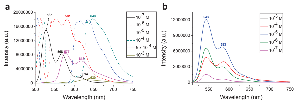
Figure 84 | a) Fluorescent spectra of PBI-PEG 7 in CD 3 CN for concentrations ranging from 10 -7 mol/L (black) up to 10 -3 mol/L (green yellow), \lambda_{\text{ex}} =483 nm; b) Fluorescent spectra of PBI-PEG 7 in D 2 O for concentrations ranging from 10 -7 mol/L (pink) up to 10 -3 mol/L (black), \lambda_{\text{ex}} =498 nm.
