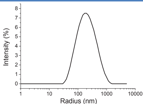
Figure 109 | Hydrodynamic radius distribution observed for PBI-6AA ([PBI-6AA] = 1 mM in D 2 O at T=25°C and \theta=173^\circ ).
