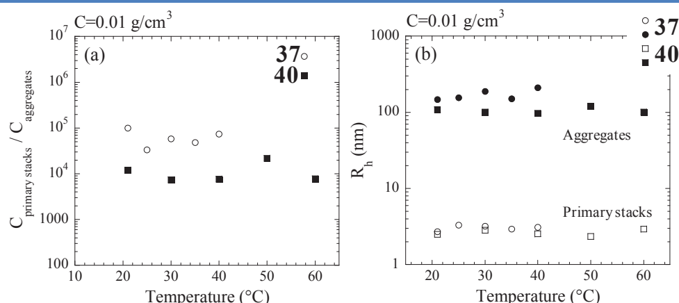
Figure 102 | Temperature dependence of (a) the ratio C_{\text{primary stacks}}/C_{\text{aggregates}} and of (b) the hydrodynamic radii R_h associated with fast (free primary stacks) and slow (aggregates) modes obtained for solutions of component 37 (circles) and 40 (squares) at C=0.01 \text{ g/cm}^3 .
