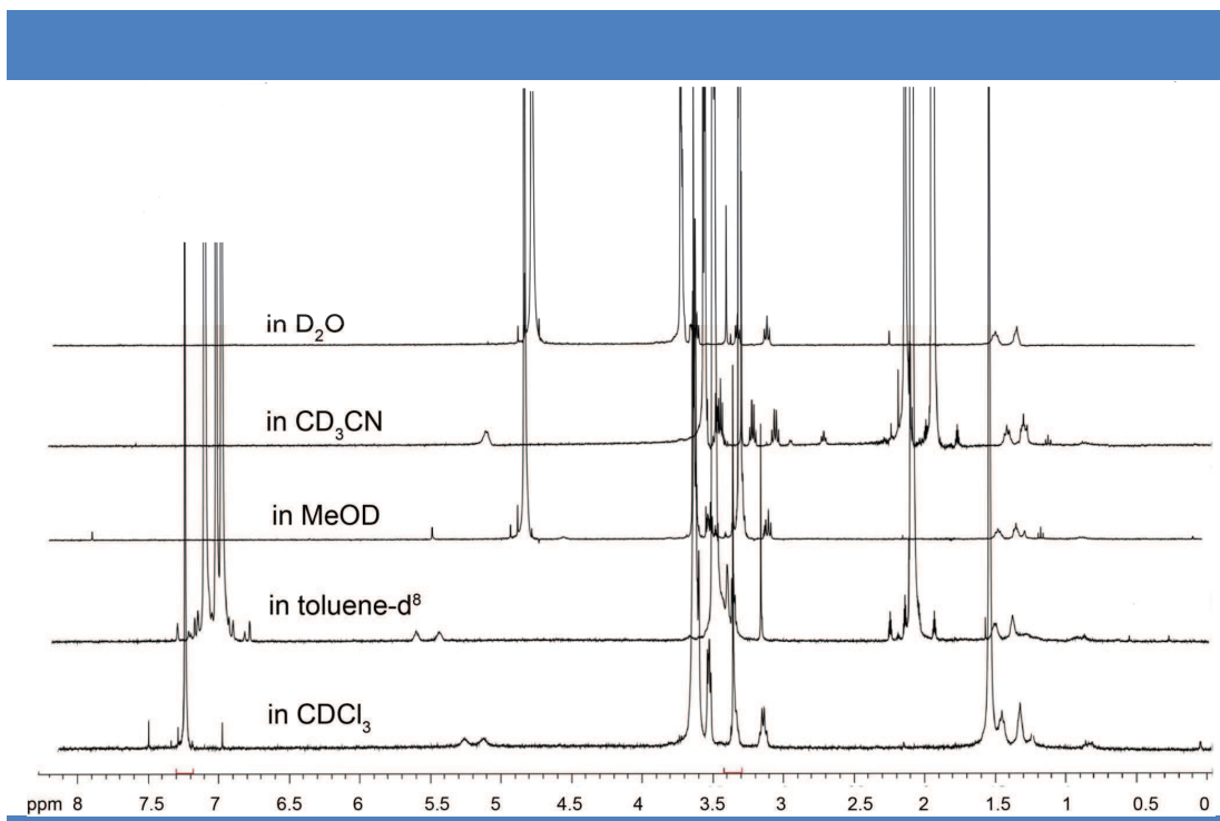
Figure 35 | ^1\text{H} NMR spectra of bisurea-PEG 7 in \text{CDCl}_3 , toluene- d^8 , MeOD, \text{CD}_3\text{CN} and \text{D}_2\text{O} at 10^{-3} M.
