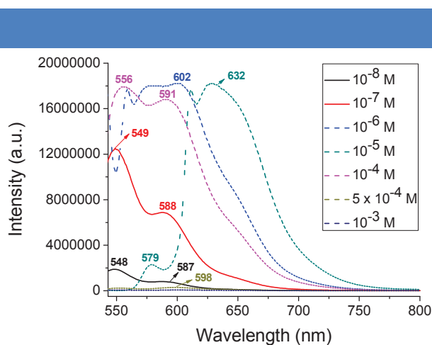
Figure 108 | Fluorescent spectra of PBI-6AA in D_2O for concentrations going from 10^{-8} mol/L (black) up to 10^{-3} mol/L (black), \lambda_{ex}=534 nm.
