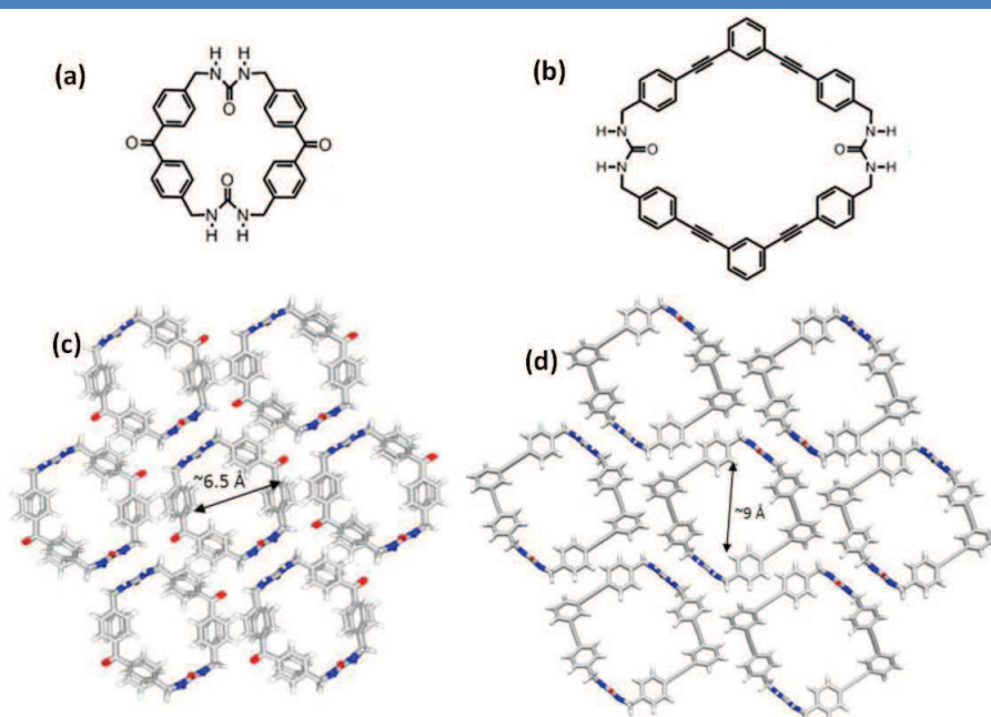
Figure 21 | a, b) Molecular structure of two bisurea macrocycles; c, d) Columnar assembly and subsequent packing of the columns affords aligned one-dimensional channels. These are viewed down the b -axis of seven hydrogen-bonded tubes of the assembled macrocycle reported in a) and b), respectively.
