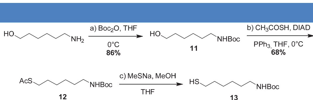
Scheme 3 | Synthesis of bifunctional linker 13
