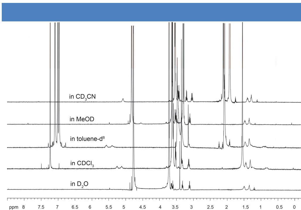
Figure 39 | ^1\text{H} NMR spectra of bisurea-PEG 16 in \text{CDCl}_3 , toluene- \text{d}^8 , MeOD, \text{CD}_3\text{CN} and \text{D}_2\text{O} at 10^{-3} M.
