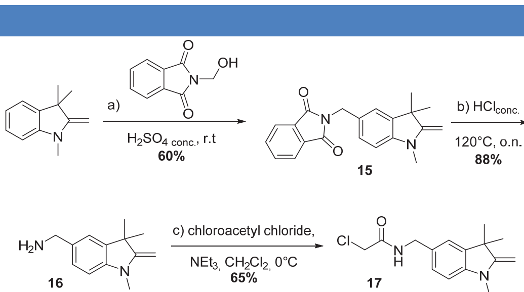
Scheme 4 | Synthesis of compound 17
