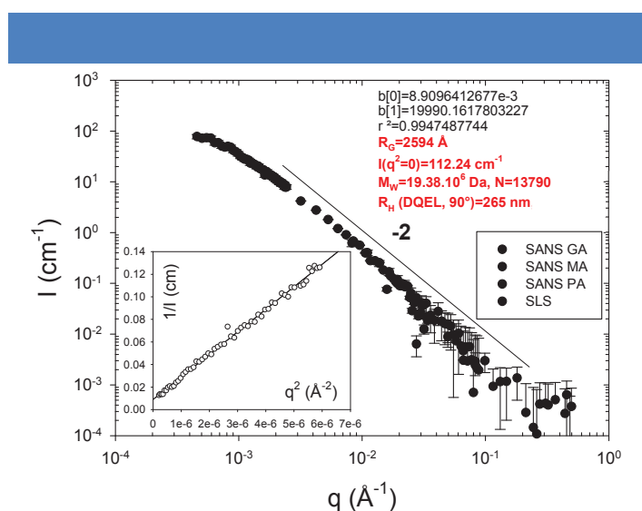
Figure 47 | SLS and SANS spectra of bisurea-6AA in D_2O at 1.43 \cdot 10^{-3}\text{ g/L} .
