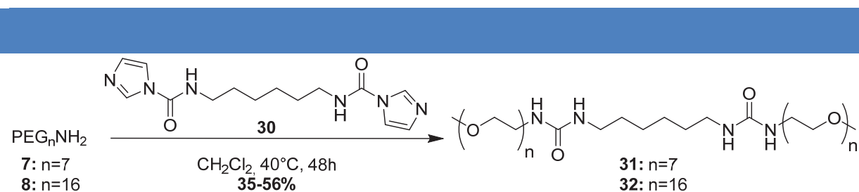
Scheme 10 | Synthesis of bisurea-PEG 7 ( 31 ) and bisurea-PEG 16 ( 32 ).
