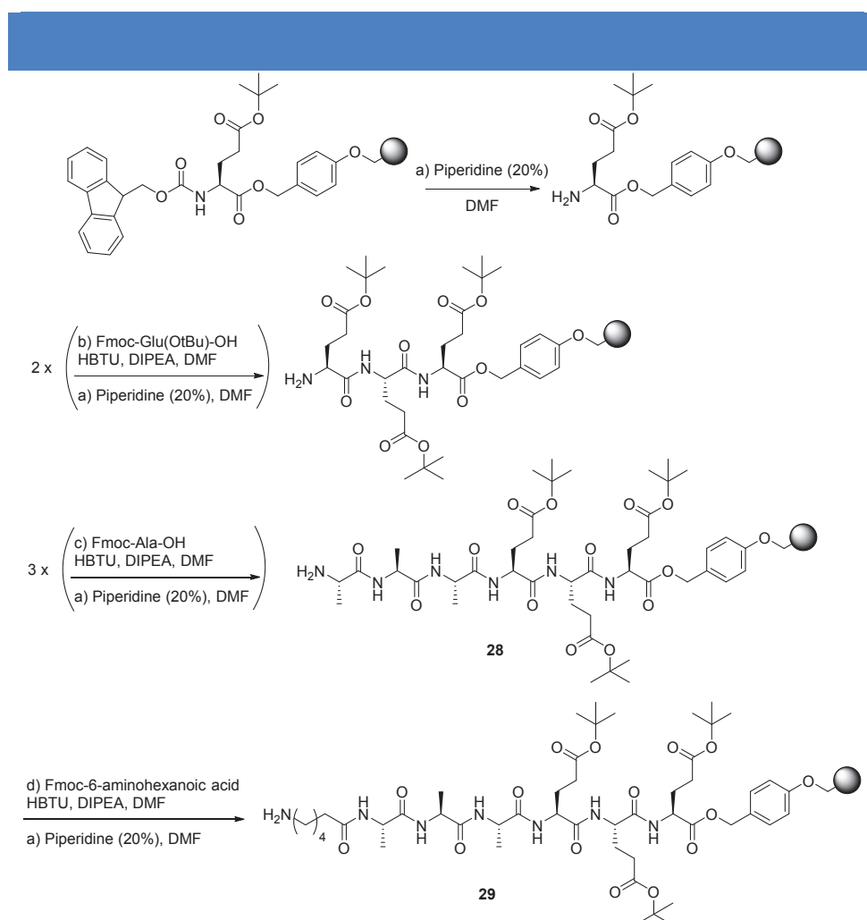
Scheme 2 | Synthesis of solid supported hexapeptide 28 and heptapeptide 29
