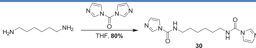
Scheme 9 | Synthesis of N,N' -1,6-hexanediylbis-1H-imidazole-1-carboxamide ( 30 )
