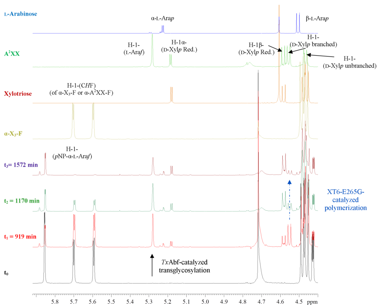
Fig. 6. ^1\text{H} NMR spectra superimposition showing the relevant anomeric H-1 signals being a feature for the monitoring of the different activities. Spectra corresponding to the different key moments reported on Fig. 5 were represented (i.e. t_0 = before trans -TxAbf (-1/+2 mutant) transglycosylation start, t_1 = before XT6-E265G addition, t_2 = before A 2 XX-containing polysaccharide precipitation, t_3 = after H-1-(CHF) total consumption).
