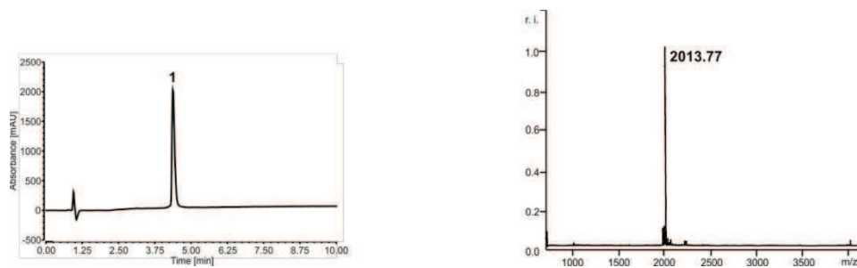
Fig.S2. HPLC and MALDI-TOF analyses of 1
