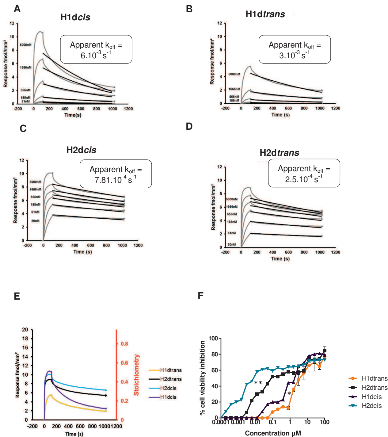
Figure 3: Different TRAIL-R2 specific peptides orientation on oligoureia helix scaffolds did not changed their biological activity. Kinetic curves of the bonding of H1dcis (A), H1dtrans (B), or H2dcis (C) and H2dtrans (D) compounds to immobilized human TRAIL-R2 (density of TRAIL-R2 was 11 fmol/mm^2 ) obtained by SPR. Compounds were tested at concentrations of 5000, 1666, 555, 185, 61 nM. The apparent k_{off} were evaluated by fitting (black curves) the post-injection phase of the curves. (E) Stoichiometries are compared by superimposing curves recorded at a 5\mu M concentration of the peptides (F) Cell viability was determined using the MTS assay as described in Figure 2 .
