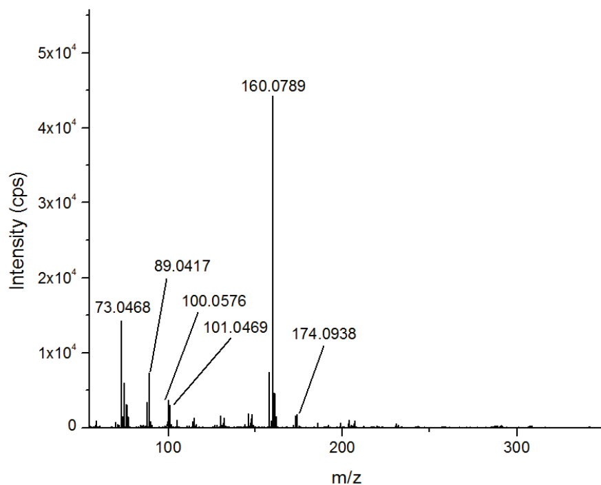
Fig.S9. Lanthionine derivative high resolution mass spectrum
