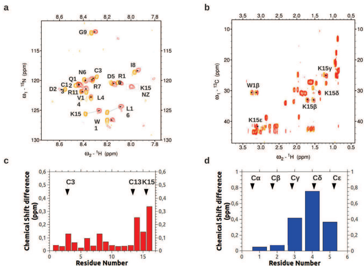
Fig.S7. Comparison of NMR data of 1 and Dim1 . a) Superimposition of the {}^1\text{H} {}^{15}\text{N} HSQC and b) {}^1\text{H} {}^{13}\text{C} HSQC spectra of 1 (yellow) and Dim1 (red). The arrows indicate the chemical shift perturbations induced by the dimerization of 1 to Dim1 . Plots of the combined chemical differences between 1 and Dim1 , in backbone amide {}^1\text{H}_\text{N} and {}^{15}\text{N} . c) versus the residue number, as well as in backbone {}^1\text{H} and {}^{13}\text{C} resonances of the branching lysine 15. d). The combined {}^1\text{H}_\text{N} and {}^{15}\text{N} shift changes were calculated as \Delta\omega (ppm) = ((\Delta^1\text{H}_\text{N})^2 + 0.1(\Delta^{15}\text{N})^2)^{1/2} . The combined {}^1\text{H} and {}^{13}\text{C} shift changes were calculated as \Delta\omega (ppm) = ((\Delta^1\text{H})^2 + 0.25(\Delta^{13}\text{C})^2)^{1/2} .
