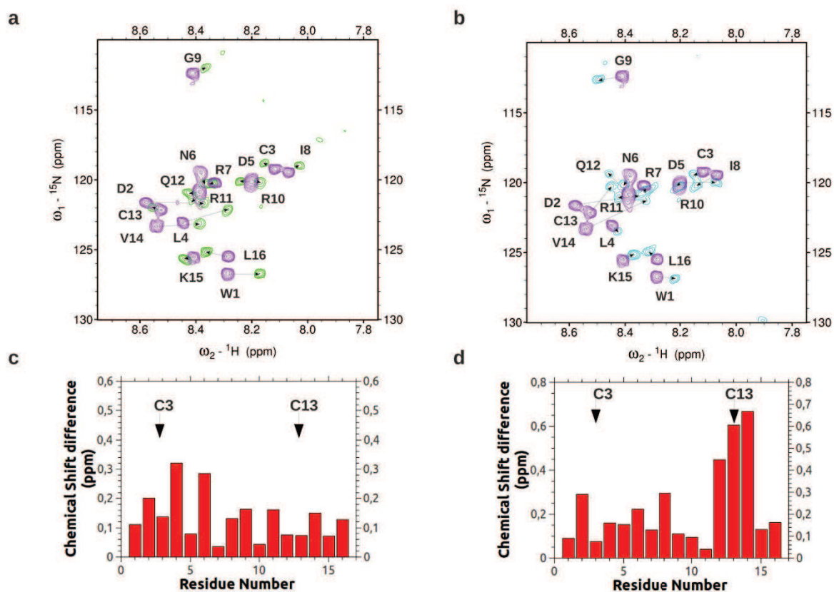
Fig.S6. Comparison of NMR data of 2b and 2c with that of 2a . Superimposition of the ^1\text{H}^{15}\text{N} HSQC spectra of a) 2b (green) and b) 2c (cyan) onto the spectrum of 2a (purple). The arrows indicate the chemical shift perturbations induced by the cysteine isomerization of 2a to 2b and to 2c . Plots of the combined chemical differences between c) 2a and 2b and d) 2a and 2c versus the residue number in backbone amide ^1\text{H}_\text{N} and ^{15}\text{N} . The combined ^1\text{H}_\text{N} and ^{15}\text{N} shift changes were calculated as \Delta\omega (ppm) = ((\Delta^1\text{H}_\text{N})^2 + 0.1(\Delta^{15}\text{N})^2)^{1/2} .
