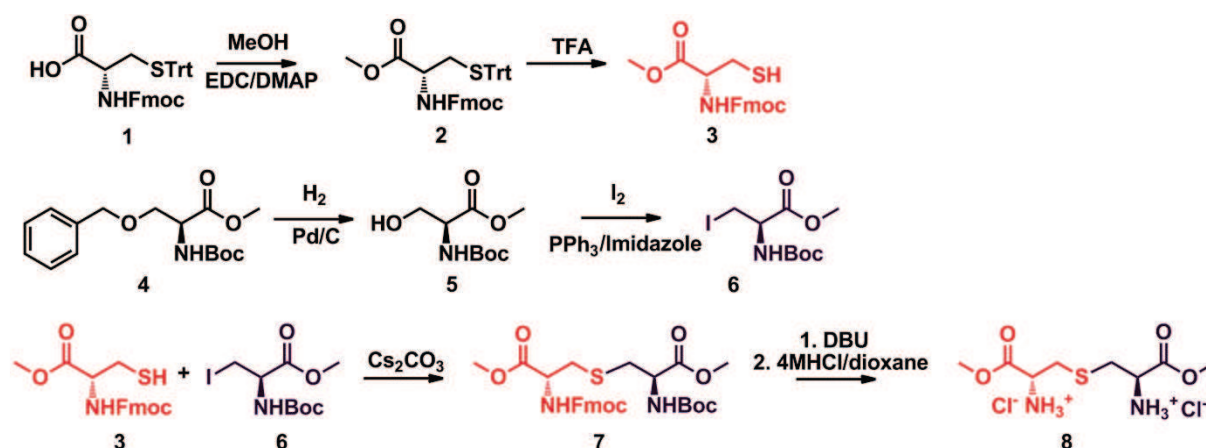
Scheme S1. Synthesis of hydrochloride of R,R -lanthionine dimethylester
