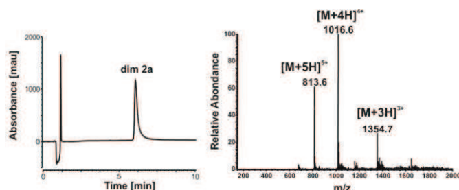
Figure 6. C_{18} HPLC trace and ESI-MS analysis of Dim2a .
