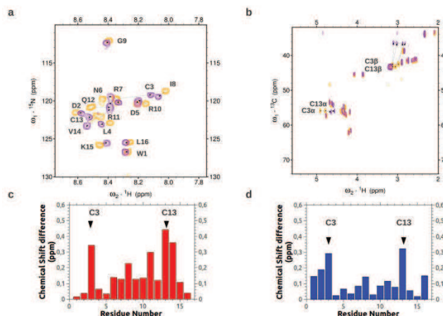
Figure 5. Comparison of 1 with 2a . Superposition of the ^1\text{H}^{15}\text{N} HSQC (a) and ^1\text{H}^{13}\text{C} HSQC (b) spectra of 1 (yellow) and 2a (purple). Plots of the combined chemical differences between 1 and 2a versus the residue number, in backbone amide ^1\text{HN} and ^{15}\text{N} (c), as well as in backbone ^1\text{H}_\alpha and ^{13}\text{C}_\alpha (d). The combined ^1\text{HN} and ^{15}\text{N} shift changes were calculated as \Delta\omega (ppm) = ((\Delta^1\text{HN})^2 + 0.1(\Delta^{15}\text{N})^2)^{1/2} . The combined ^1\text{H}_\alpha and ^{13}\text{C}_\alpha shift changes were calculated as \Delta\omega (ppm) = ((\Delta^1\text{H}_\alpha)^2 + 0.25(\Delta^{13}\text{C}_\alpha)^2)^{1/2} . The arrows indicate the chemical shift perturbations induced by the desulfurization of 1 to 2a .
