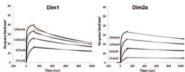
Figure 7. Kinetic curves of disulfide-bridged cyclic peptides Dim1 and desulfurized peptide Dim2a binding to immobilized human DR5 (density of 65 fmol/mm 2 ). Compounds were injected at concentrations 5000, 2500, 1250, 625 and 312 nM. The response is expressed in fmol/mm 2 (1000RU = 1 mg/mm 2 ). The fitted post-injection phases are in grey.
