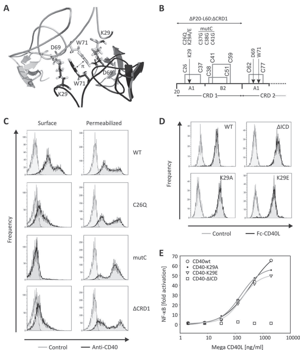
FIGURE 2. CD40-CRD1 is required for normal surface expression. A , detail of the CD40 dimer model in the region of CRD1-CRD1 interaction, showing side chains of K 29 , D 69 , and W 71 . B , schematic representation of the CRD1 domain of CD40 with disulfide bridges highlighted. Mutations tested are indicated. C , flow cytometry analysis of HEK293 cells transfected with untagged WT or mutant CD40 constructs. Staining was performed with an anti-CD40 antibody in permeabilized or nonpermeabilized (surface) conditions. D , flow cytometry analysis of different CD40-HEK293 stable cell lines used in this study. Staining was performed with Fc-CD40L followed by anti-human Fc-PE. E , dose response of CD40L in a NF- \kappa B luciferase activity assay in different CD40-expressing HEK cell lines (CD40-WT, CD40-K29A, CD40-K29E, and CD40- \Delta ICD).
