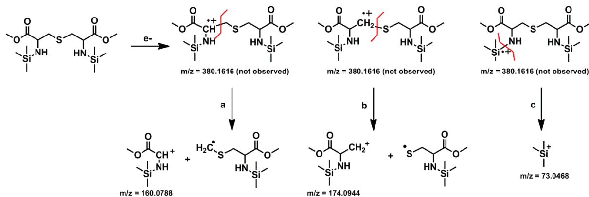
Fig. S10: Fragmentation analysis
