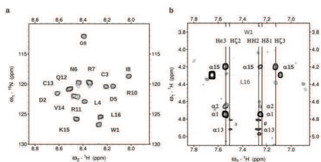
Figure 3. NMR analysis of 1 . a) Annotated 1 H 15 N HSQC spectrum of 1 acquired at 293K, pH 5.85 in 95% H 2 O/5% D 2 O. The assignment of the peaks is indicated with the amino acid one letter code followed by the residue number. b) Aromatic-backbone proton region of a 300 ms NOESY spectrum acquired at 293K, pH 5.85 in 95% H 2 O/5% D 2 O. Straight lines along the F1 dimension indicate the aromatic side-chain proton resonances of the tryptophan W1. NOE cross peaks with the backbone residue protons are boxed and assigned. The C-terminal amide group of the residue L16 is identified by a horizontal line
