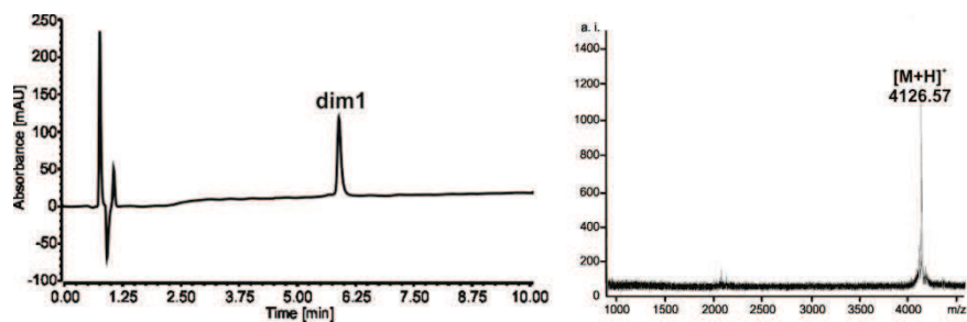
Fig.S4. HPLC and MALDI-TOF analyses of Dim1 .
