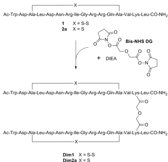
Scheme 2. Dimerization of cyclic peptides 1 and 2a with the diglycolic linker Bis-NHS DG .
