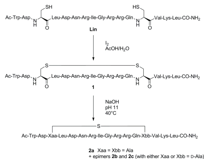
Scheme 1. Synthesis of cyclic peptide 1 and its desulfurization to thioether peptide analogues 2 .
