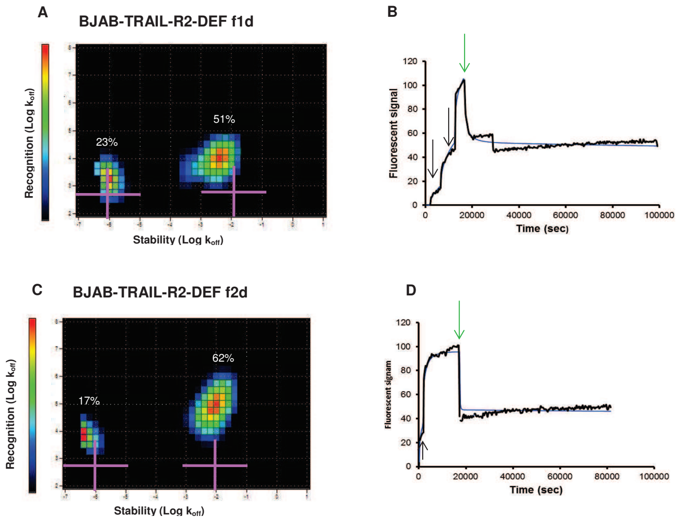
Figure 6: LT binding measurements of the interaction between 1d or 2d on BJAB-TRAIL-R2-DEF. Interaction Maps (A and C) were calculated from real time LT binding measurements (B and D) of the interaction between divalent peptides f1d (A and B) and f2d (C and D) and BJAB deficient for the expression of TRAIL-R2. The contribution of each interaction to the signal (%) is indicated in white in the maps. The experimental curves are in black and the fitted curves in blue (right hand panels). The black arrows correspond to the addition of 10 then 30 nM of peptides 1d (upper-right panel) and 10nM for 2d (lower right panel) to the cells. The green arrows indicate the removal of peptides.
