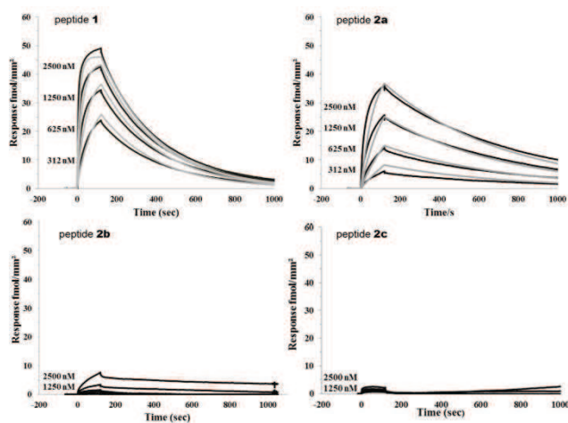
Figure 2. Kinetic curves of disulfide-bridged cyclic peptides 1 and desulfurized peptide 2a-2c binding to immobilized human DR5 (density of DR5 is 65 fmol/mm 2 ). All compounds were tested at concentrations 5000, 2500, 1250, 625 and 312 nM. The response is expressed in fmol/mm 2 (1000RU= 1mg/mm 2 ). The fitted curves are in grey.
