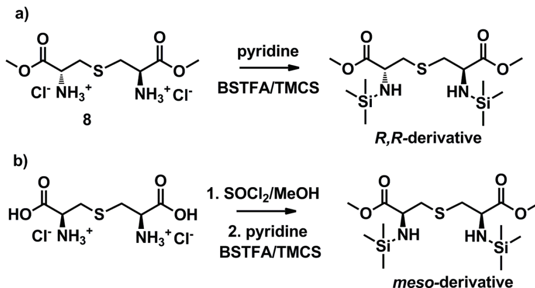
Scheme S2. Derivatization of lanthionines: a) R,R -lanthionine b) meso -lanthionine
