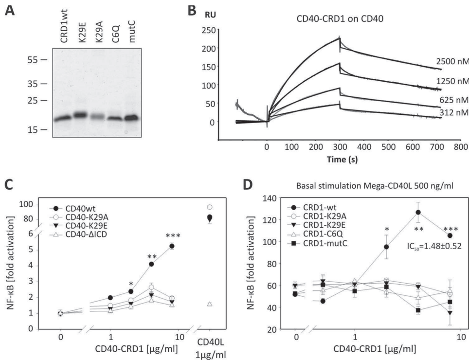
FIGURE 4. Recombinant CD40-CRD1 binds to CD40 and potentiates CD40L activity. A , purified CD40-CRD1, CRD1-K29E, CRD1-K29A, CRD1-C6Q, and CRD1-mutC (20 μg of protein/lane) were resolved by SDS-PAGE and stained with Coomassie Blue. B , Biacore sensorgram of CD40-CRD1 binding to the entire extracellular domain of CD40. C , luciferase reporter assay for NF-κB activity in different CD40 HEK cell lines (CD40wt, CD40-K29A, CD40-K29E, and CD40-ΔICD) treated with recombinant soluble CD40-CRD1. Untreated cells are shown on the left, and Mega-CD40L-stimulated cells are shown on the right. D , luciferase reporter NF-κB assay in HEK CD40 cell line treated with 500 ng/ml CD40L and increasing concentrations of recombinant soluble CD40-CRD1, CRD1-K29A, CRD1-K29E, CRD1-C6Q, and CRD1-mutC. Mean values with S.E. (error bars) of three independent experiments are shown (*, p < 0.05 ; **, p < 0.01 ; ***, p < 0.001 ).
