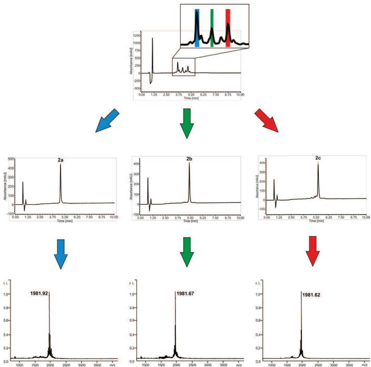
Fig.S3. HPLC and MALDI-TOF analyses of crude and purified diastereoisomers obtained after desulfurization of 1 .
