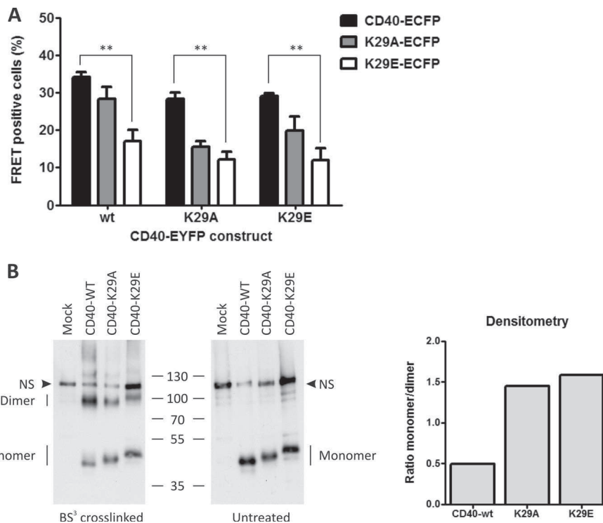
FIGURE 3. Mutations of lysine 29 disrupt CD40 self-assembly. A , cytometric FRET analysis was performed of CD40 interaction with WT CD40, CD40-K29A, or CD40-K29E, using both ECFP and YFP fusion combinations. Mean values with S.E. (error bars) of three independent experiments are shown (**, p < 0.01 ). B , CD40 stable cell lines (WT, K29A, and K29E) were treated or not with the nonpermeable chemical cross-linker BS 3 . CD40 was then detected by Western blotting with an anti-CD40 antibody. Densitometry analysis is shown on the right as a ratio between monomeric and dimeric receptors. NS, nonspecific signal.
