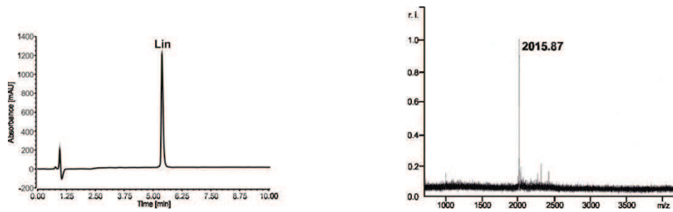
Fig. S1. HPLC and MALDI-TOF analyses of Lin
