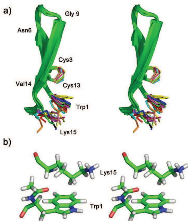
Figure 4. NMR-derived molecular model of peptide 1 . a) Stereoview of the ten superimposed lowest energy structures. The strands of the \beta -hairpin structure are shown as green ribbons. The side chains of the disulphide bridge C3/C13 and of the hydrophobic cluster W1/K15 are shown as lines. b): Stereoview of the hydrophobic cluster between the side-chains of the tryptophan W1 and the lysine K15.
