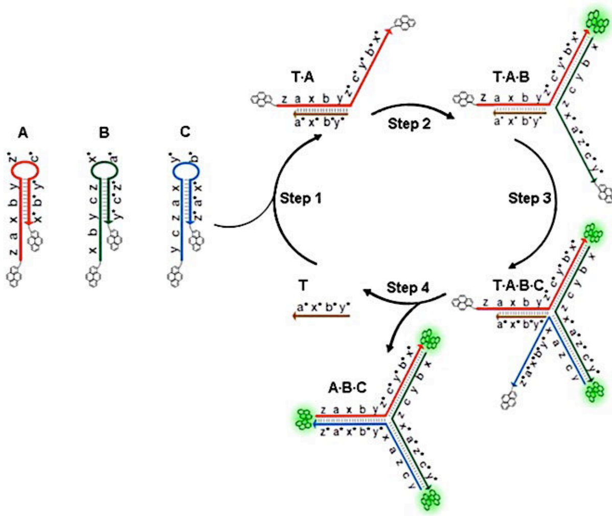
Fig. 9.3 Schematic representation of an enzyme-free nucleic acid amplified detection (T = Target DNA, A = Probe A, B = Probe B, C = Probe C). The presence of target catalyzes the formation of hybridized structures that lead to the formation of pyrene excimer couples, whose fluorescence signal is detected. Reprinted with permission from Z. Qing, X. He, J. Huang, K. Wang, Z. Zou, T. Qing, et al. Anal. Chem. 2014 , 86 , 4934-4939. Copyright (2014) American Chemical Society.
