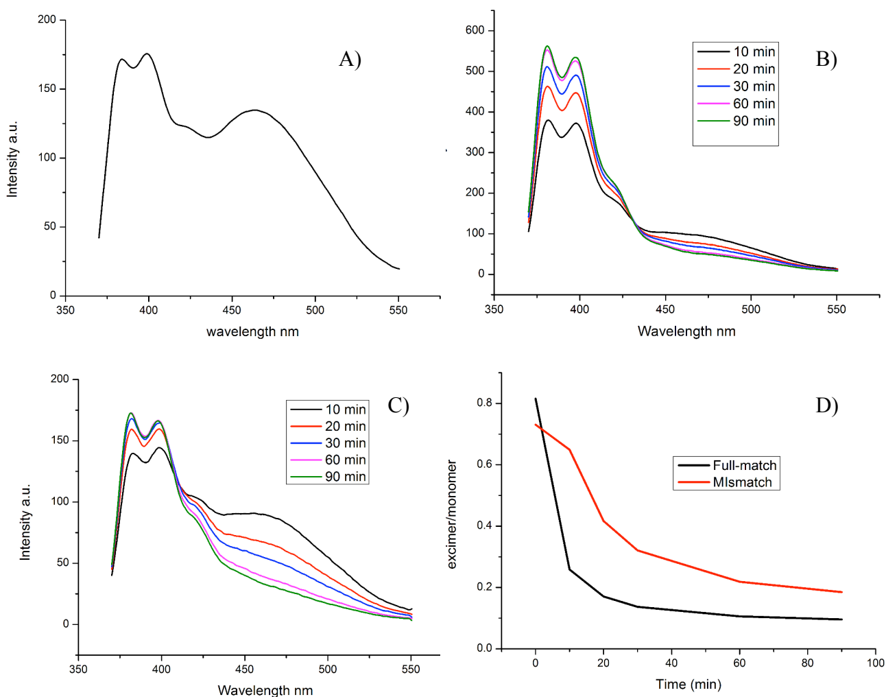
Fig. 9.15 A) Fluorescence emission spectrum of a 1 μM aqueous solution of the dual-pyrene modified PNA probe, before addition of the target DNA, 40° C. B) Emission spectrum profiles over time when adding the full match sequence to the PNA switching probe solution at 40° C. C) Same emission profile over time in presence of a single mismatch sequence. D) Kinetics of the interaction between the PNA probe and the DNA sequences (black line = full match, red line = mismatch), expressed as the excimer/monomer intensity ratio as function of time.
