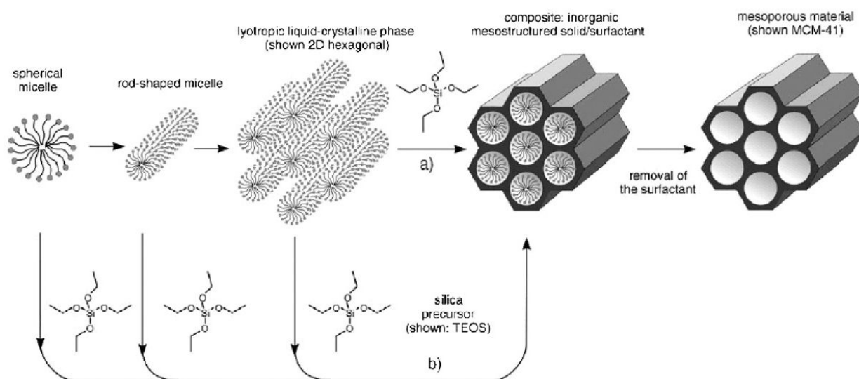
Fig. 2.9 Scheme of synthesis of MSNPs with CTAB surfactant micelles as template. Adapted from F. Tang, L. Li, D. Chen, Adv. Mater. 2012 , 24 , 1504-1534. Copyright © 2012 WILEY-VCH Verlag GmbH & Co. KGaA, Weinheim
