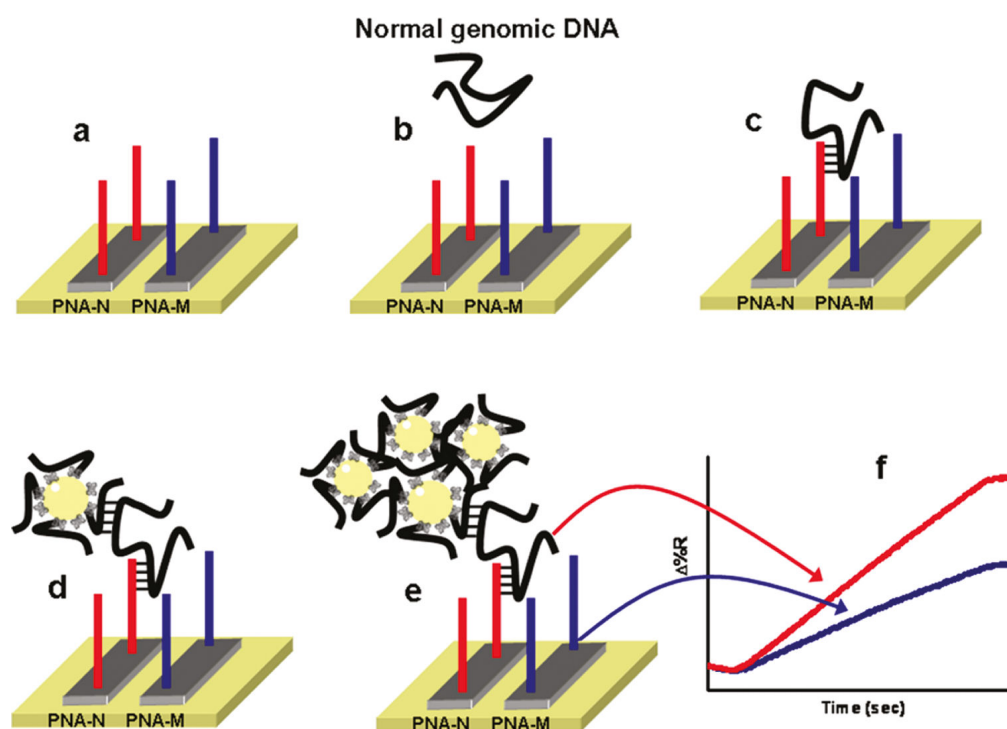
Fig. 1.18 Schematic description of the nanoparticle-enhanced SPR strategy used to detect a normal \beta^N/\beta^N , a heterozygous \beta^{39}/\beta^N , and a homozygous \beta^{39}/\beta^{39} genomic DNA. In order to simplify the pictorial representation only specifically adsorbed DNA is shown. Nonspecifically adsorbed DNA is also present on the surface and contributes to generate the SPR-detected signal. PNA-N and PNA-M probes specifically recognize the normal \beta -globin and the mutated \beta^{39} -globin genomic sequences, respectively. Reprinted with permission from R. D'Agata, G. Breveglieri, L.M. Zanoli, M. Borgatti, G. Spoto, R. Gambari, Anal. Chem. 2011 , 83, 8711-8717. Copyright (2011) American Chemical Society.
