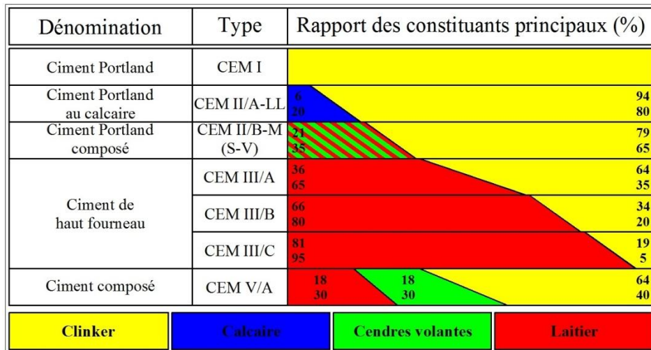
Figure 1 : compositions des ciments courants (Roux, 2008)
