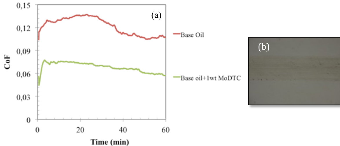
Fig. 5.38. Friction behavior of a-C:H:Si:O DLC/ a-C:H:Si:O DLC tribo-pairs configuration lubricated by MoDTC-containing base oil (a). Friction wear track on the silicon-doped DLC flat coupon (b). Value to be compared to Figure 5.1 and 5.2.
