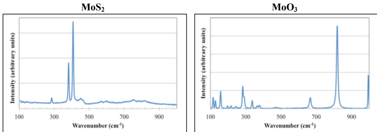
Fig 2.11. Raman spectra of MoS 2 and MoO 3 reference materials.
