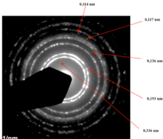
Fig. 5.18. SAED pattern of the tribofilm showing the extra spots present in the pattern (a). Some experimental Miller indices may match the graphite theoretical values (JCPDS 00-026-1079)(b).
