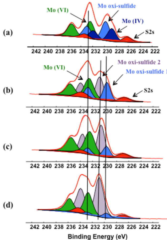
Fig 2.10. XPS High-resolution Mo3d spectra changes in the tribofilm as a function of the oxidation time considering three contributions for fresh sample (a), 2 hours aged (b), 5 hours aged (c) and 8 hours aged (d) oil.
