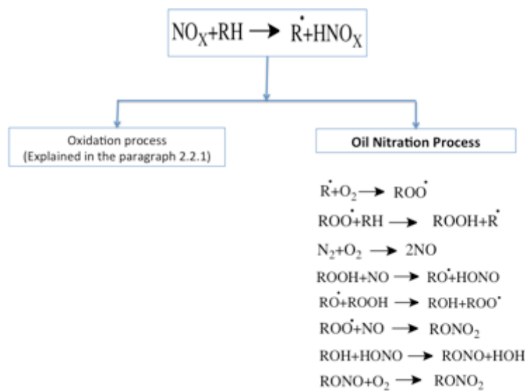
Fig 1.2. Nitration mechanisms
