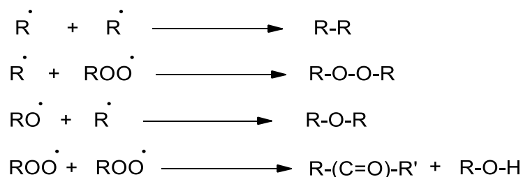
Scheme 1.5. Termination reactions producing a variety of products – a) Long chain hydrocarbons. b) Dialkyl peroxides. c) Ethers. d) Ketones and alcohols.
