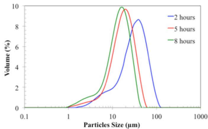
Fig. 4.6. DLS distribution for the particles collected from the aged oils. The oil samples were submitted to 30 minutes of ultra-sonic bath.
