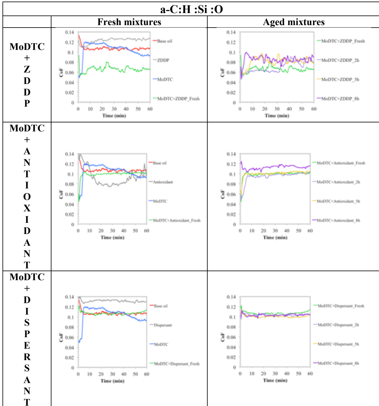
Fig. 6.10. Friction behavior for MoDTC/Antioxidant and MoDTC/Dispersant mixtures, fresh and aged for a-C:H:Si:O DLC/steel contact
