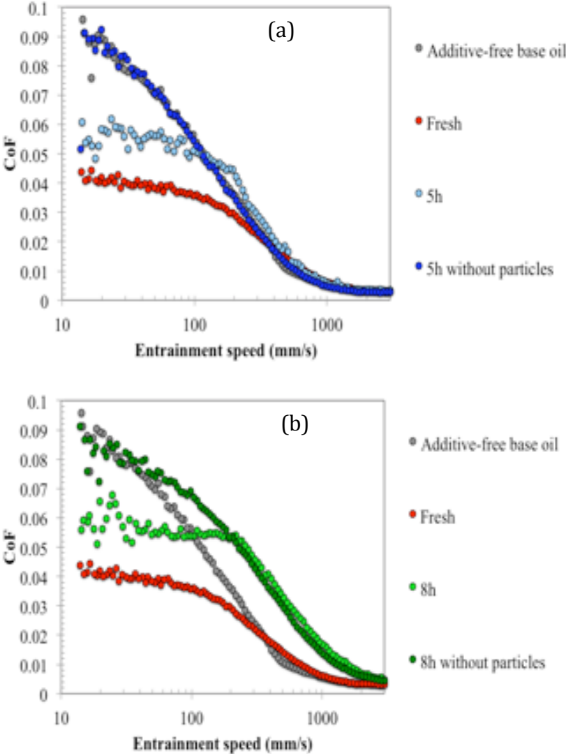
Fig. 4.13. Stribeck curves obtained with aged oils, with and without particles (Step 2) after 5 hours (a) and 8 hours (b) of degradation process. Tests carried out using MTM tribometer.
