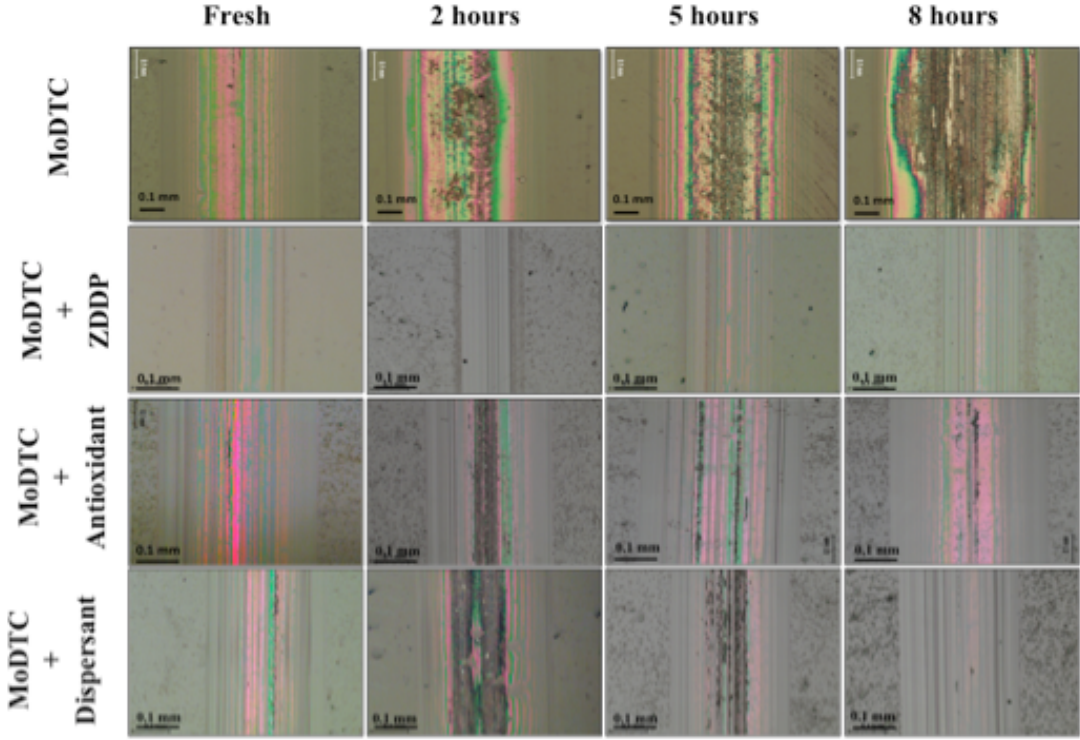
Fig. 6.11. Optical images for the a-C:H:Si:O DLC coated flats tested with fresh and aged samples.
