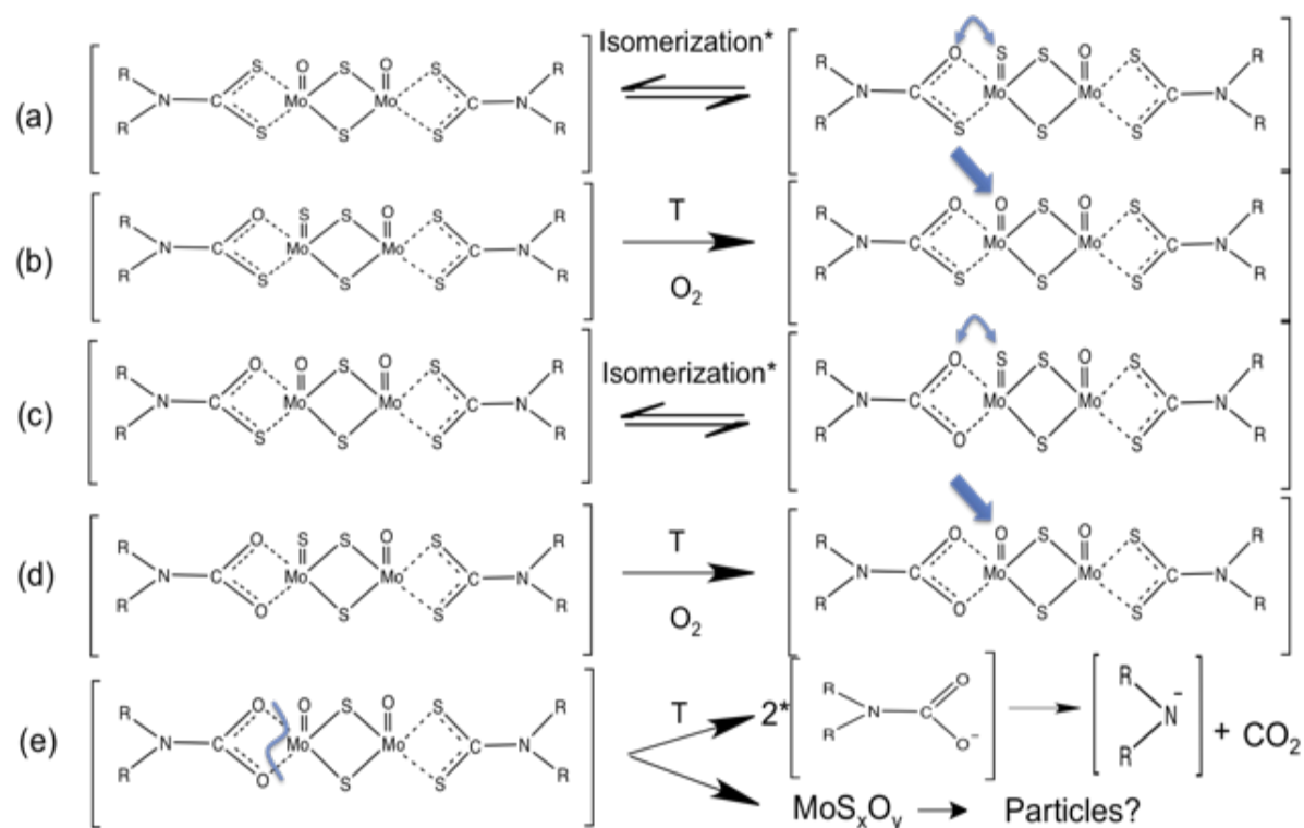
Fig 3.13. Supposed chemical pathway followed by MoDTC molecule during thermo-oxidative degradation
