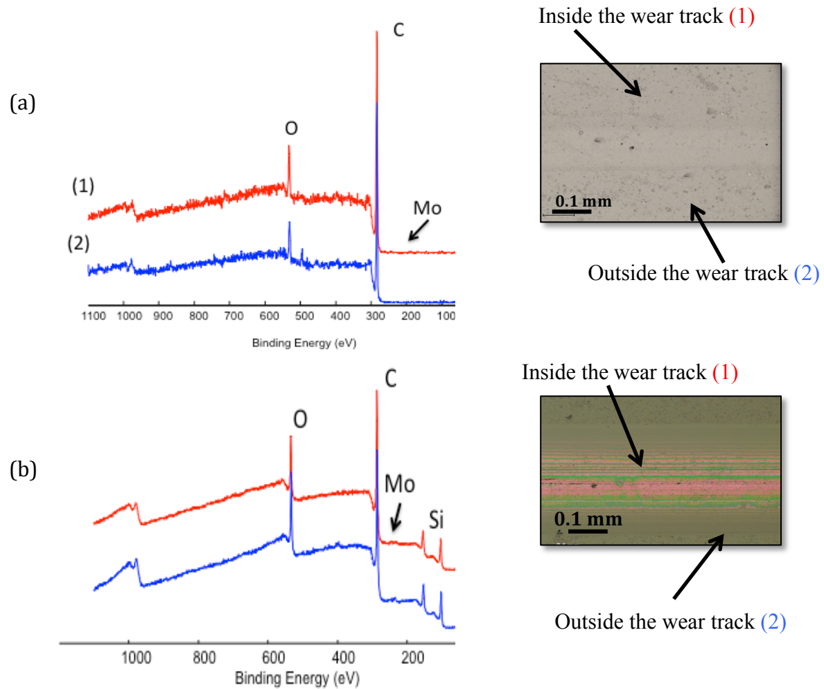
Fig 5.5. Survey spectra recorded on a-C:H DLC coated flat (a) and silicon-doped DLC (b) lubricated by fresh MoDTC-containing oil.
