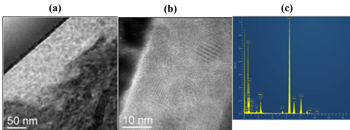
Fig 2.16. TEM micrographs of the cross-section of the tribofilm formed on steel after friction test using 1% wt MoDTC in mineral base oil aged for 8 hours, where no MoS 2 sheet structures are visible (a) and the iron oxides particles are present in the tribofilm (b, c).
