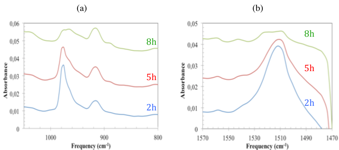
Fig 3.12. The resultant absorbance spectra after subtraction with the fresh oil in the area (800-1040) \text{ cm}^{-1} corresponding to Mo=O bond (a) and in the area (1470-1570) \text{ cm}^{-1} corresponding to C-N bond (b).
