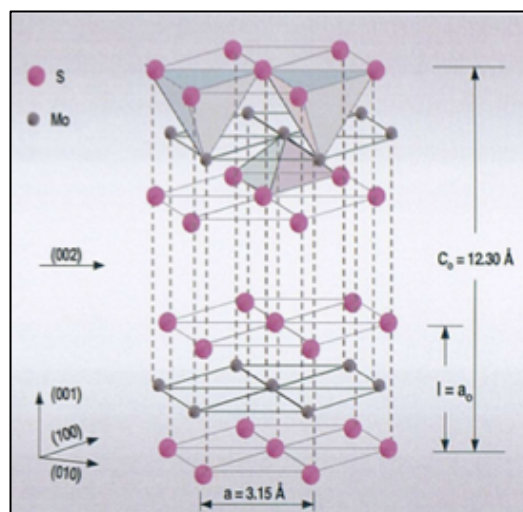
Figure 1.4. Lamellar crystal structure of 2H-MoS 2 .
