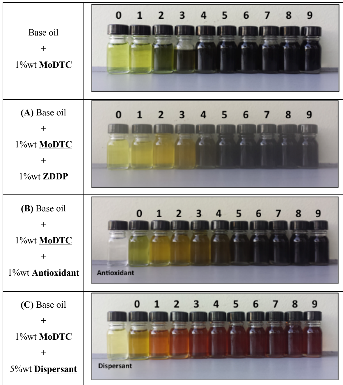
Fig. 6.3. Visual inspection of the three mixtures analyzed in this chapter.
