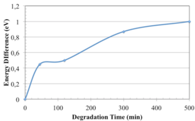
Fig 2.9. Chemical shift in the binding energy of the Mo (IV) line between fresh and aged oil as a function of oxidation time.
