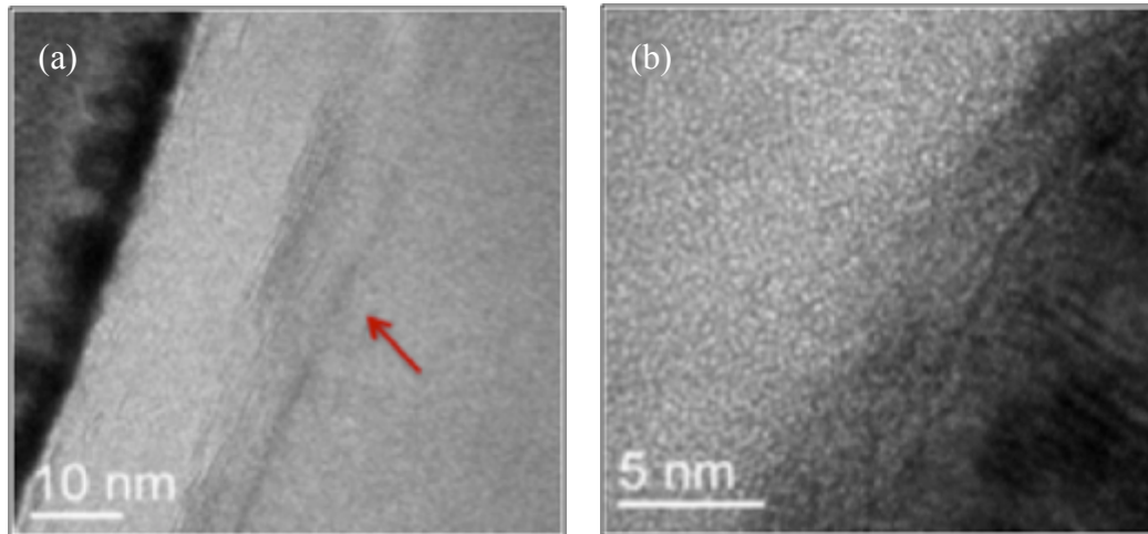
Fig 2.15. TEM micrographs of the cross-section of the tribofilm formed on steel after friction test using 1% wt MoDTC in mineral base oil aged for 2 hours, showing the well-aligned MoS 2 sheets located on top part of the tribofilm (a) while no chevron-like structure of S-Mo-S sandwich was visible (b).
