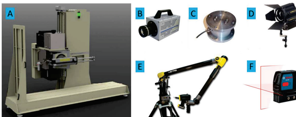
Figure 2-6 : Main instrumentation on the ex-vivo protocol. A. Impact Machine (LF Technologies France), B. High-speed recording camera (FASTCAM SA3, Photron, Japan). C. Six-axis sensor (105515TF, Humanetics, Germany). D. projector (400D, Dedolight, Germany). E. Laser arm scan (Nikon, Japan). F. Positioning laser.
