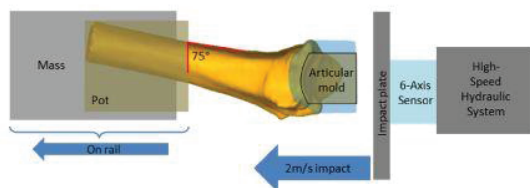
Figure 1. Schema of the impact test.
