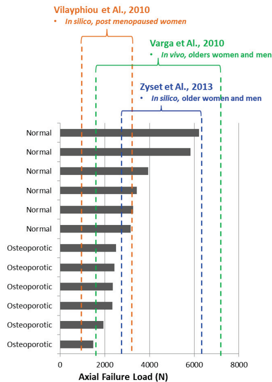
Figure 3-8 : Comparison of the failure load obtained with values from similar studies in literature (Vilayphiou et al. 2010; Varga et al. 2010; Zysset et al. 2013). the grey bars represents the current values.
