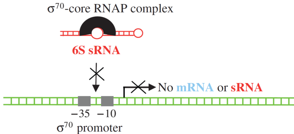
Figure 17: RNA polymerase interacts with 6S sRNA in E.coli . RNA synthesis by the “ \sigma^{70} -core RNA polymerase” complex (black). 6S sRNA (red) sequesters the polymerase complex during nutrient limitation (stationary phase of growth), and restrain gene expression to the ones controlled by an alternative \sigma factor [From (Pichon & Felden 2007)].
