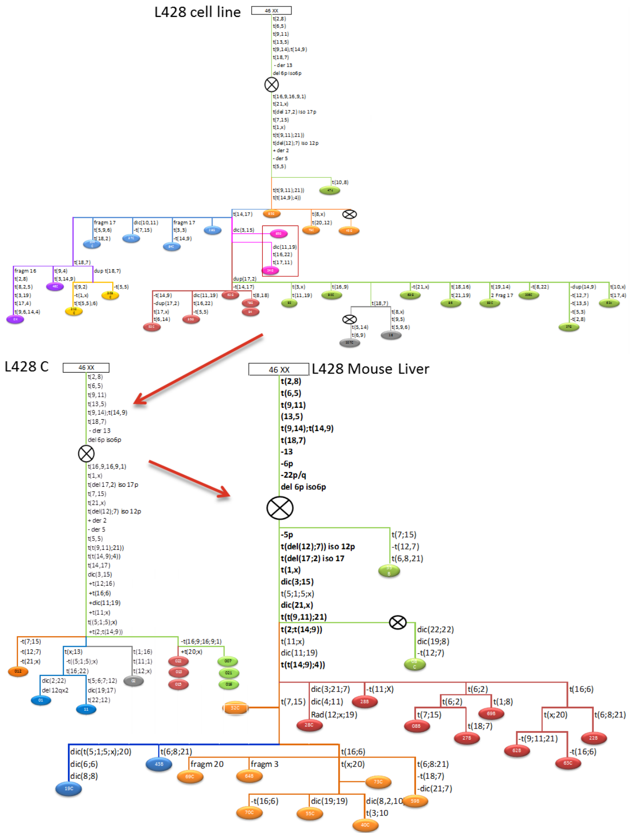
Figure 7: Trees of L428 cell line, cell derived from methylcellulose and cell derived from mice.
