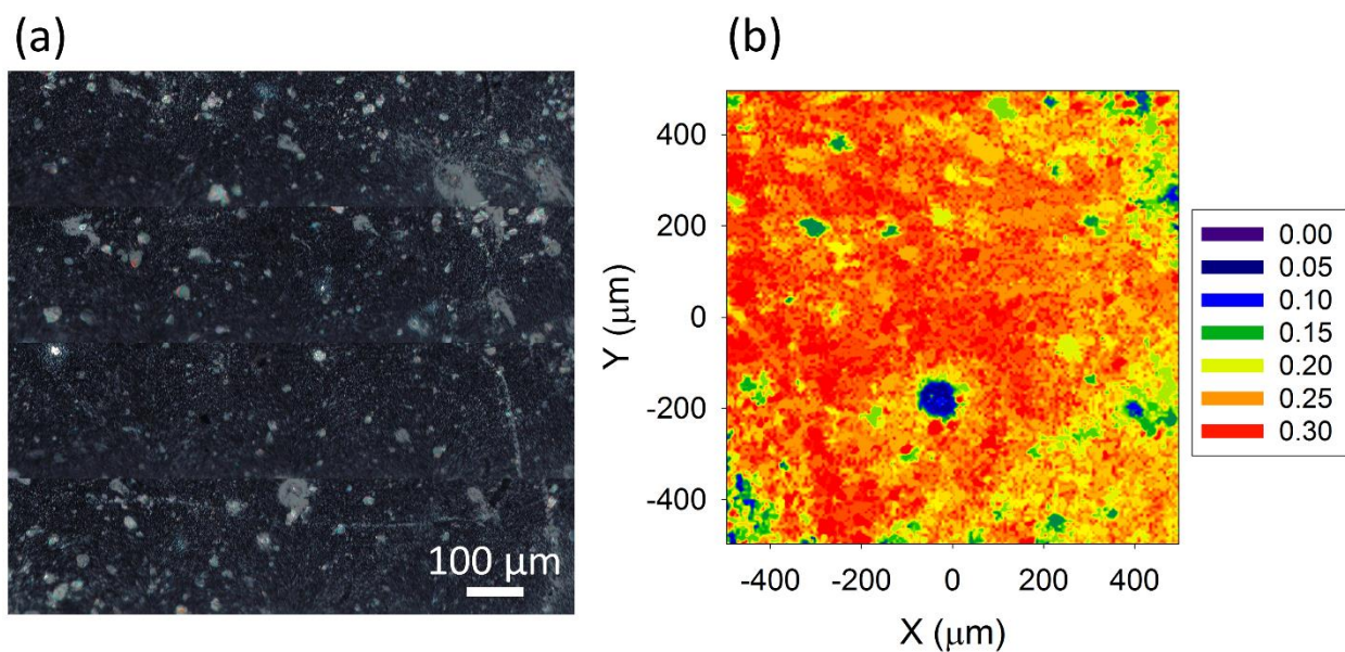
Figure 4.11. Optical micrograph taken inside the poled area after it reacted (a) IR map showing the distribution of the intensity of the water band around 3200\text{ cm}^{-1} (b)
