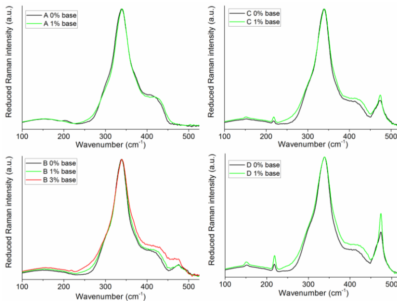
Figure 5.9. Reduced Raman spectra of the base glasses (black) compared to the glasses with addition of 1% sodium sulfide (green) and 3% sodium sulfide (red)
