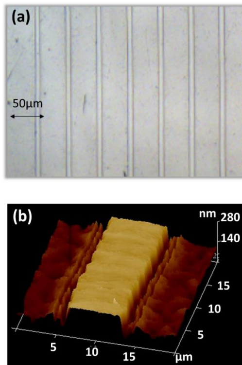
Figure 3.4. Optical micrograph (a) and topology image of the glass surface after thermal poling (b)
