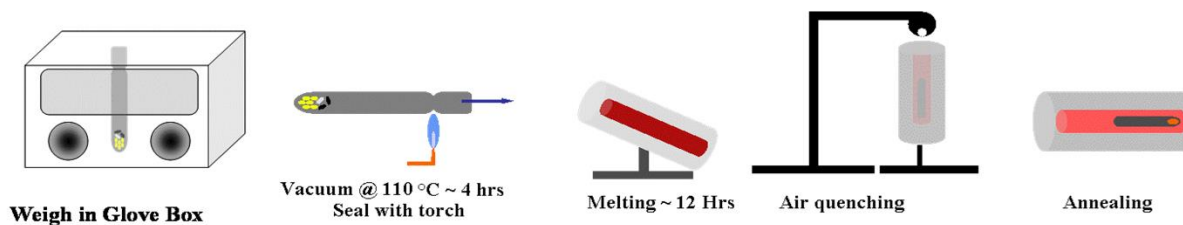
Figure 2.1. Preparation steps of a chalcogenide glass
