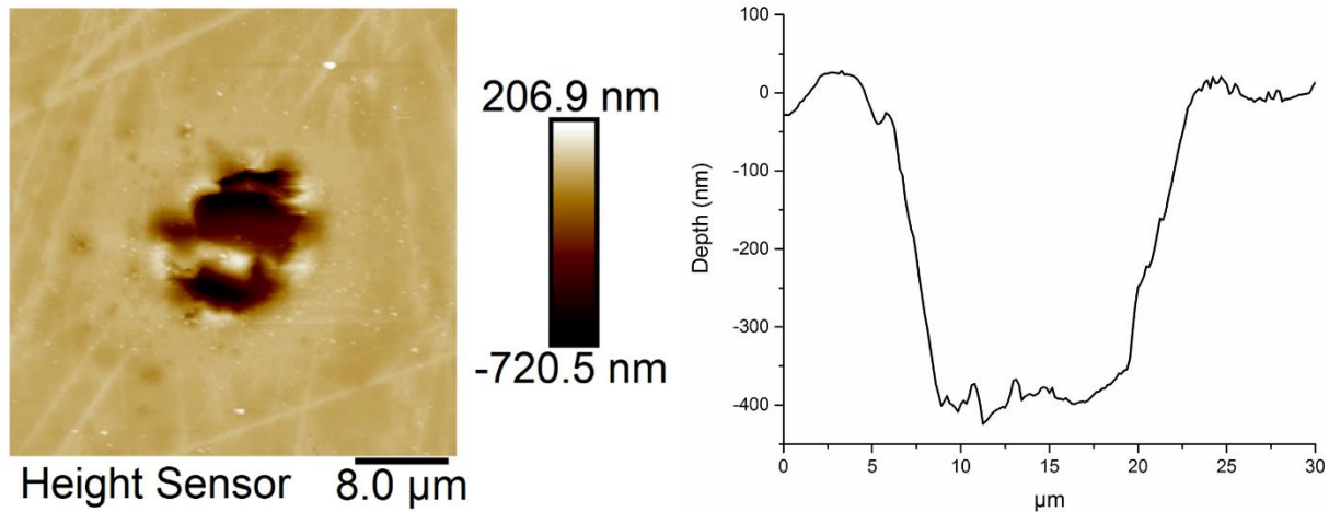
Figure 4.23. AFM measurements measured across an irradiated spot (left) and corresponding topology profile (right)
