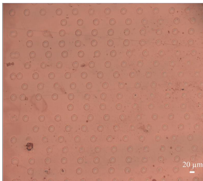
Figure 5.25. Points imprinted on the glass surface using an electric field induced imprinting process on compositions B - 1% Na 2 S (a) and B - 3% Na 2 S (b)
