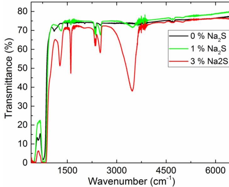
Figure 5.4. Transmittance spectra in the infrared of the B series with 0, 1 and 3% of Na 2 S.
