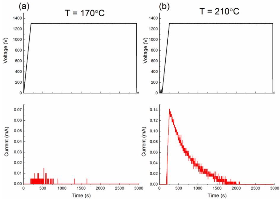
Figure 5.14. Voltage profile (top) and current measured across the sample (bottom) thermally poled at 170°C (a) and 210°C (b)
