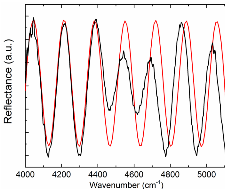
Figure 5.39. Interference fringes measured in IR reflectance spectroscopy on the poled sample B-1% (black) along with a fit (red)
