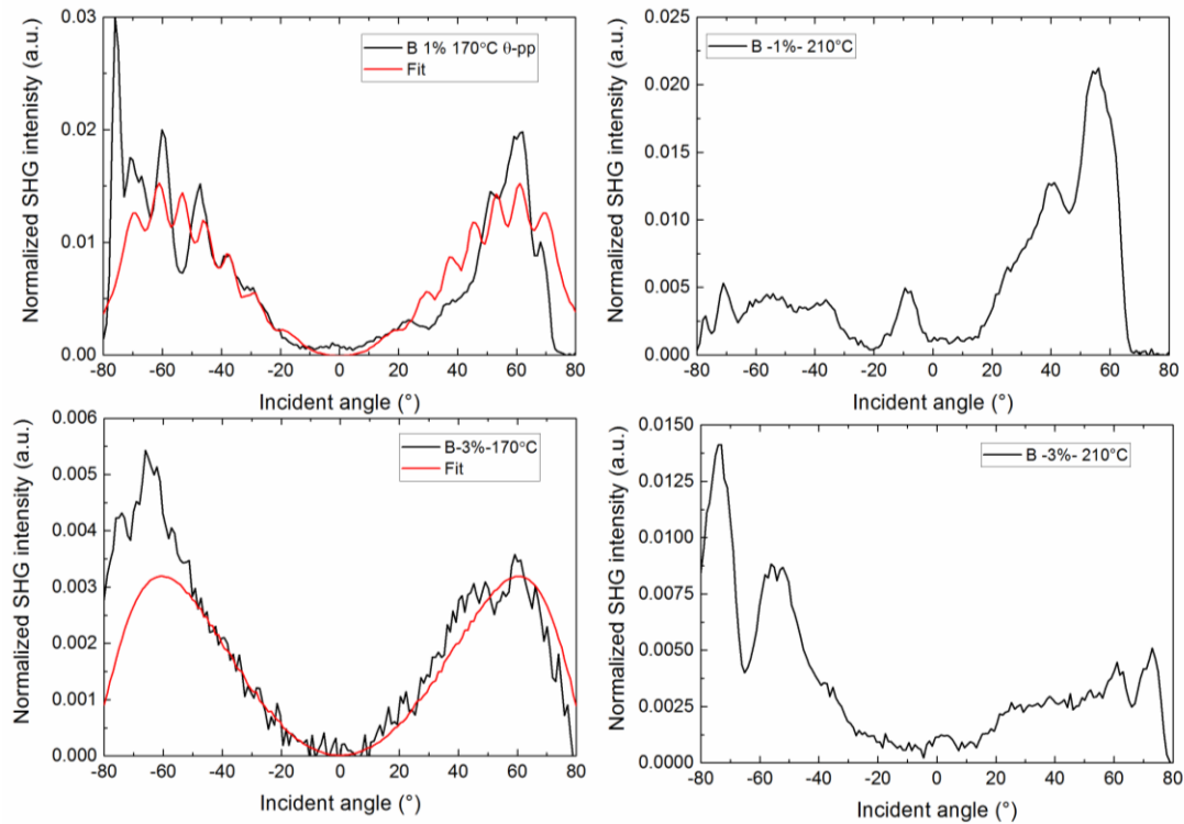
Figure 5.17. \theta -scans recorded for glass B-1% Na 2 S poled at 170°C and 210°C (top row) and glass B-3% Na 2 S poled at 170°C and 210°C (bottom row), fits are presented in red when possible
