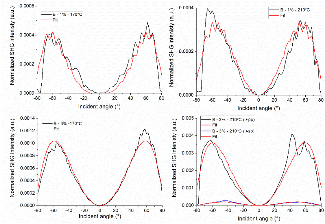
Figure 5.18. Maker fringes measured all Na-rich glasses two months after thermal poling
