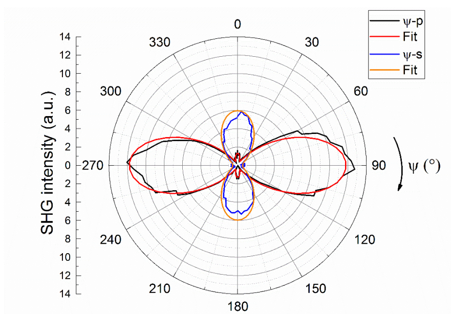
Figure 5.24. Polar plot of \psi -scans recorded at normal incidence along with fit obtained for an electro-optical contribution along x and y
