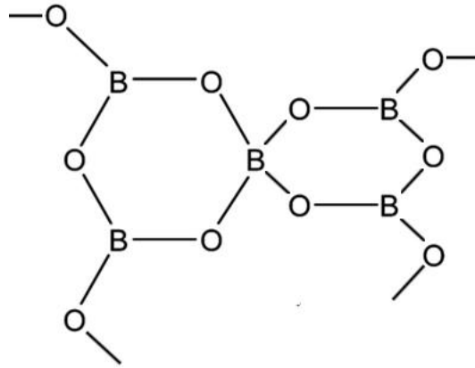
Figure 4.4. Schematic representation of a pentaborate group
