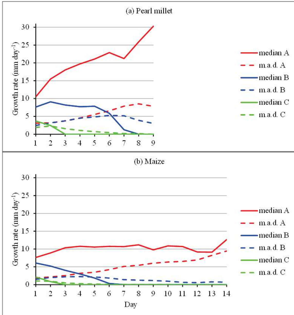
Figure 2-4: Daily median growth rate (and associated mean absolute deviation –m.a.d.–) for (a) pearl millet and (b) maize.
