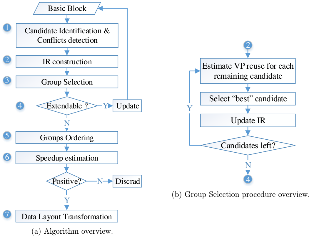
Figure 4.3 – Holistic SLP algorithm flow diagram.
