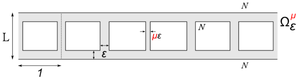
Figure 1.2: Perturbed domain ( \mu < 1 )
