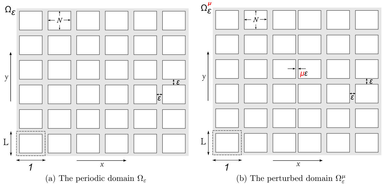
Figure 4.1: The purely periodic domain \Omega_\varepsilon and the perturbed domain \Omega_\varepsilon^\mu .
