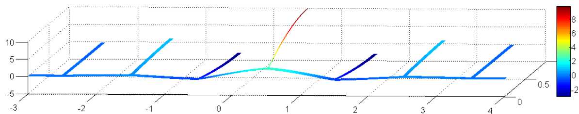
(b) \varepsilon = 0.06 , \lambda_1 \approx 1.40
