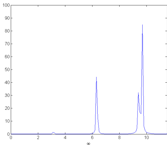
(a) error\_T_{01} for k = 0, h = 0.1
