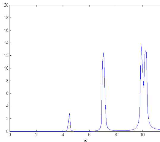
(b) error\_T_{00} for k = 1, h = 0.1
