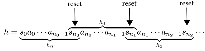
Figure 4: Factorizing an infinite history into weaknesses
