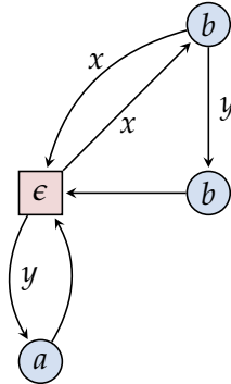
Figure 6: An arena for the game with payoff f
