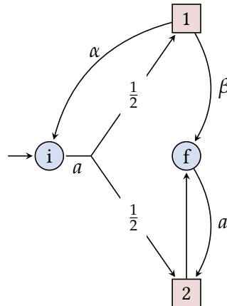
Figure 13: A half-blind game
