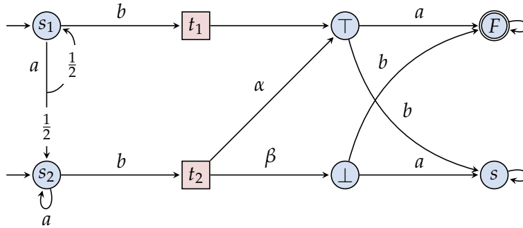
Figure 21: A gadget
