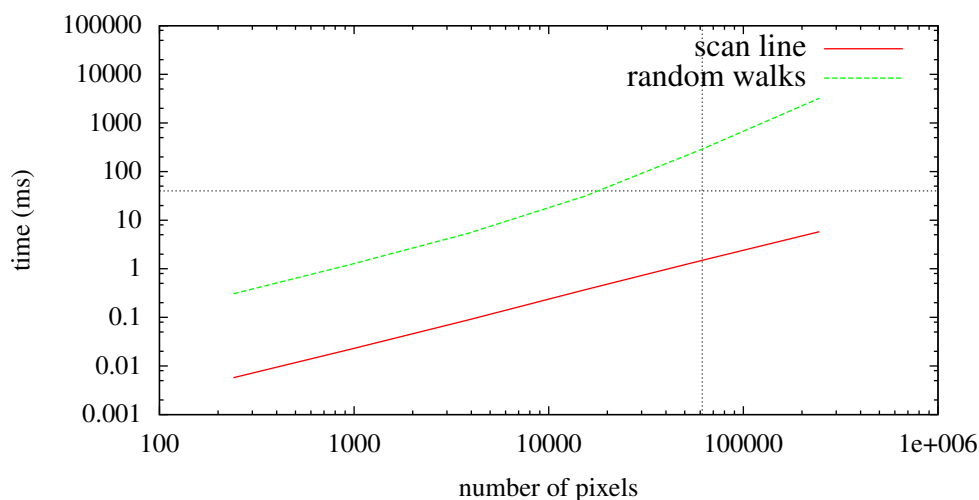
Figure 1.24 – Computation time for the random walks confidence map and the scan line integration methods. For reference, the dotted lines correspond to a standard acquisition rate of 25 frames per second and a prescan image size of 480 \times 128 . Both axes are in logarithmic scale.
